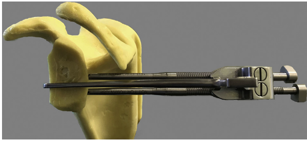
Fig 7. Jig fixation. The guide arm and tip have been placed in the desired position on the left anterior glenoid. The 2 drill guide bullets have been inserted and ratcheted down onto the posterior glenoid.
