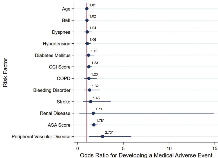
Figure 1. Multimodal logistic regression analysis showing adjusted odds ratio scatter chart for the associations between development of a medically related adverse event and Charlson Comorbidity Index (CCI), American Society of Anesthesiologists (ASA) physical classification system, or demographic and comorbidity variables shown to be significant. *Indicates of significance the risk factor in the multimodal model at the P = .05 level. BMI, body mass index; COPD, chronic obstructive pulmonary disease.
