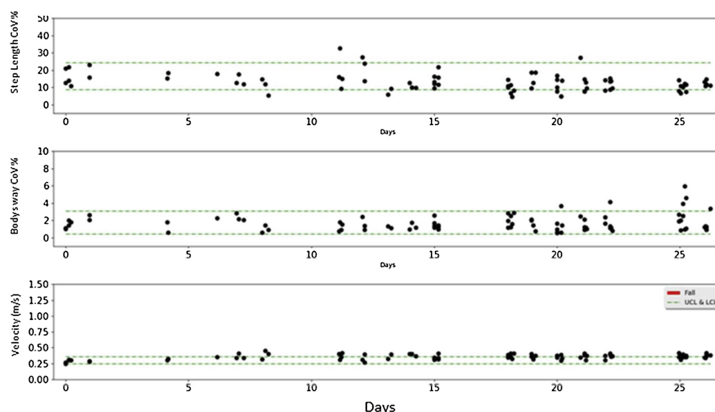
Fig. 2. Control charts illustrating gait data from the feasibility study in two subjects (A + B). Red lines indicate falls and green lines are control limits ( \pm 2 standard deviations) based upon the first seven days of baseline data. CoV = Coefficient of variability, calculated as the standard deviation of the gait quantity within one gait episode divided by the mean of the gait quantity within the same gait episode.
