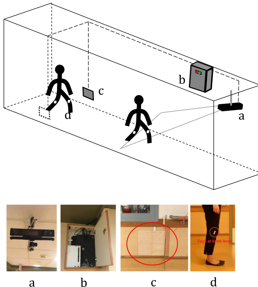
Fig. 1. AMBIENT set-up in the hallway of the Geriatric Psychiatry unit at TRI-UHN. AMBIENT set-up includes a Kinect sensor (a), a control box (b), and two RFID antennas (c). Two RFID tags (d) were attached to participants' clothing at knee level.
