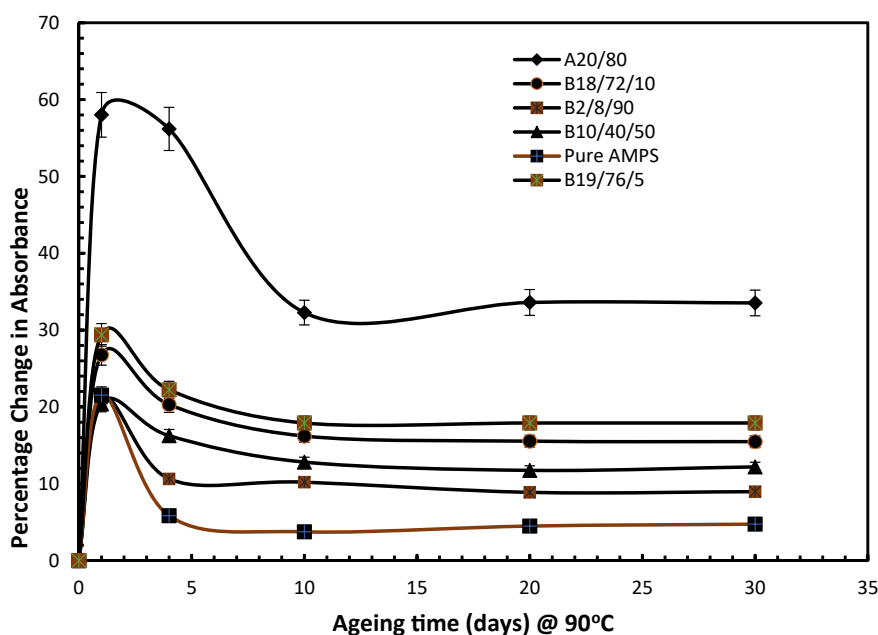
Fig. 11. Percentage change in amide absorbance polymer weight ratio composition at 90 °C and 200,000 ppm TDS. (symbol A and B representing the PAM: PVP mixture and the PAM:PVP:AMPS mixtures, respectively).
