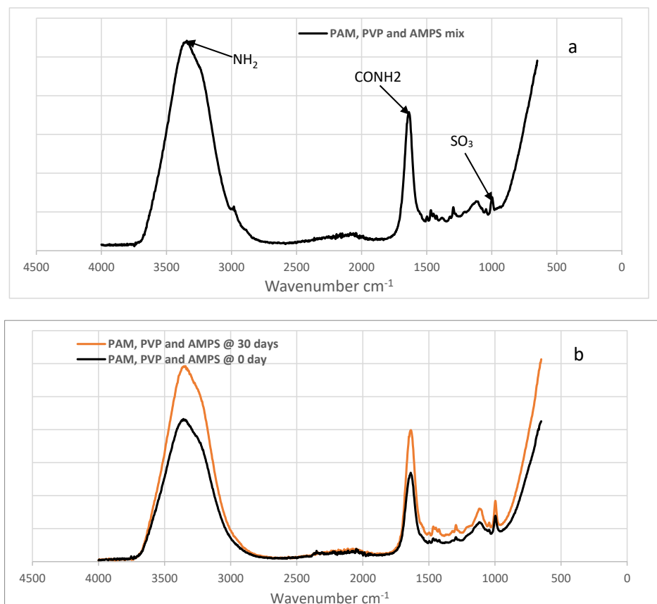
Figure 9. FT-IR absorbance spectra for (9a) PAM, PVP and AMPS (9b) Comparative PAM, PVP and AMPS mix samples at time 0 and 30 days.
