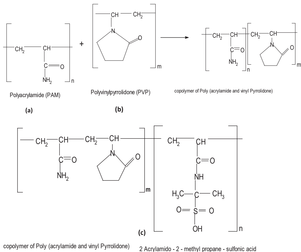
Fig. 1. Molecular structure of (a) PAM, (b) PVP and (c) AMPS.
