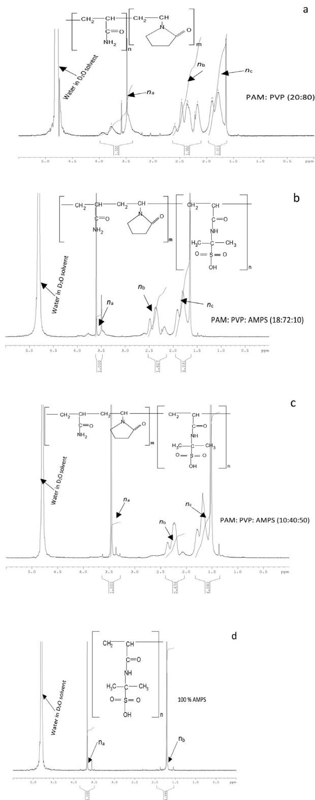
Fig. 12. 1 H NMR spectra for the four selected weight ratio of polymer mixtures of PAM:PVP and PAM:PVP:AMPS in brine with TDS of 200,000 ppm at 90 °C. In this figure, 12a is for A 20/80 wt%, 12b is for B18/72/10 wt%, 12c is for B10/40/50 wt% and 12d is for 100% AMPS (symbol A and B representing the PAM: PVP mixture and the PAM:PVP:AMPS mixtures, respectively). na, nb and nc present amide group, methylene amide group and methylene group, respectively.
