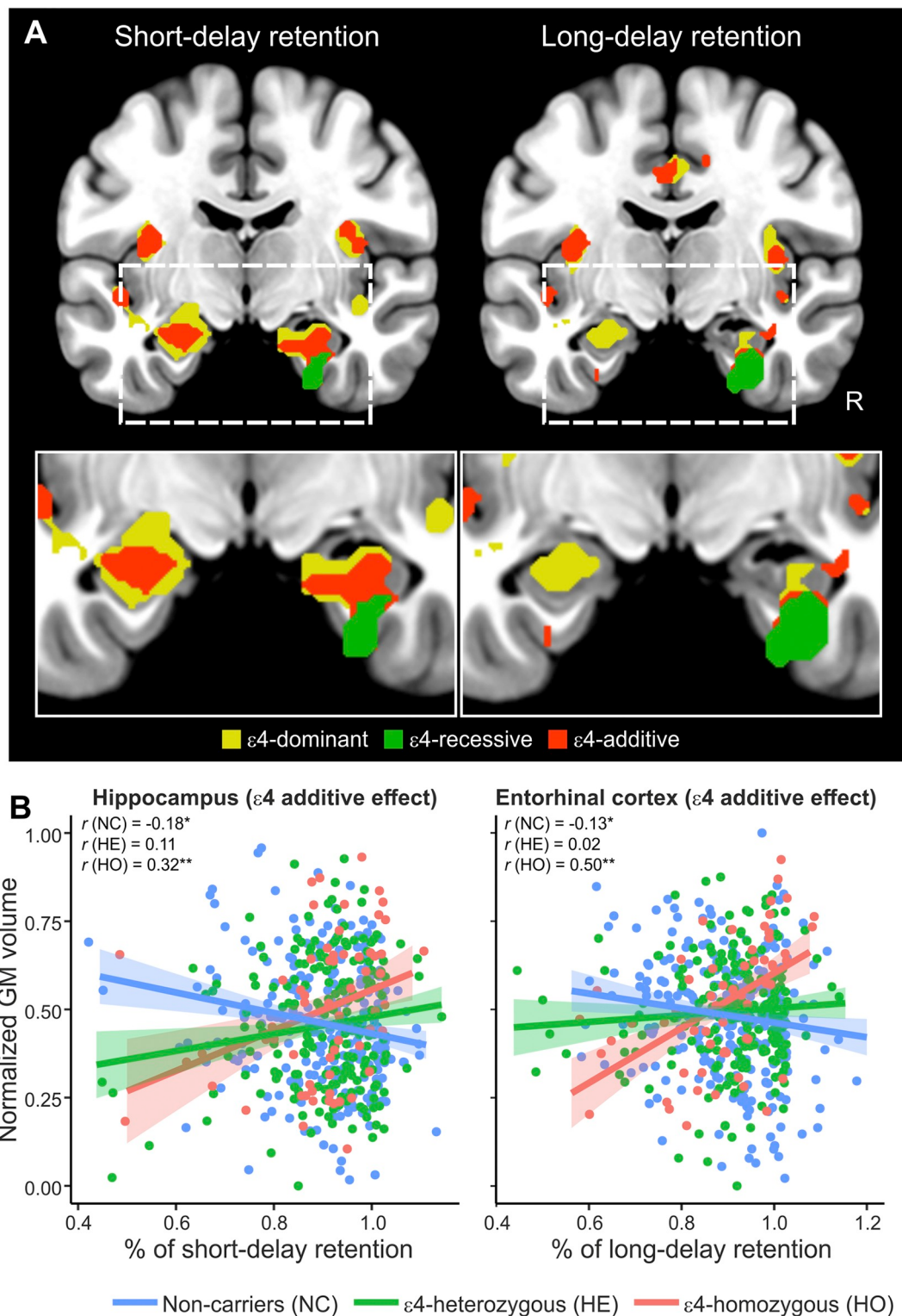
Fig. 3. Effects of the APOE-ε4 risk variant in modifying the association between memory retention and regional gray matter volume.
