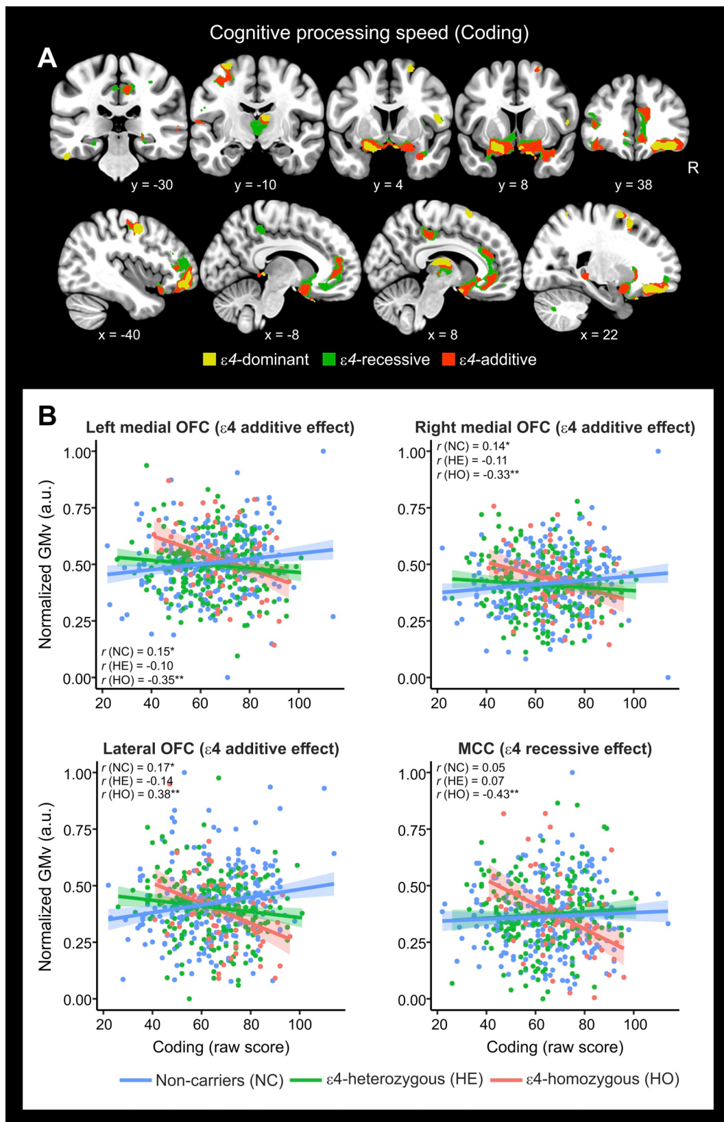
Fig. 4. APOE- \epsilon 4 risk variant modulated the associations between cognitive processing speed (CPS) and gray matter volume.
