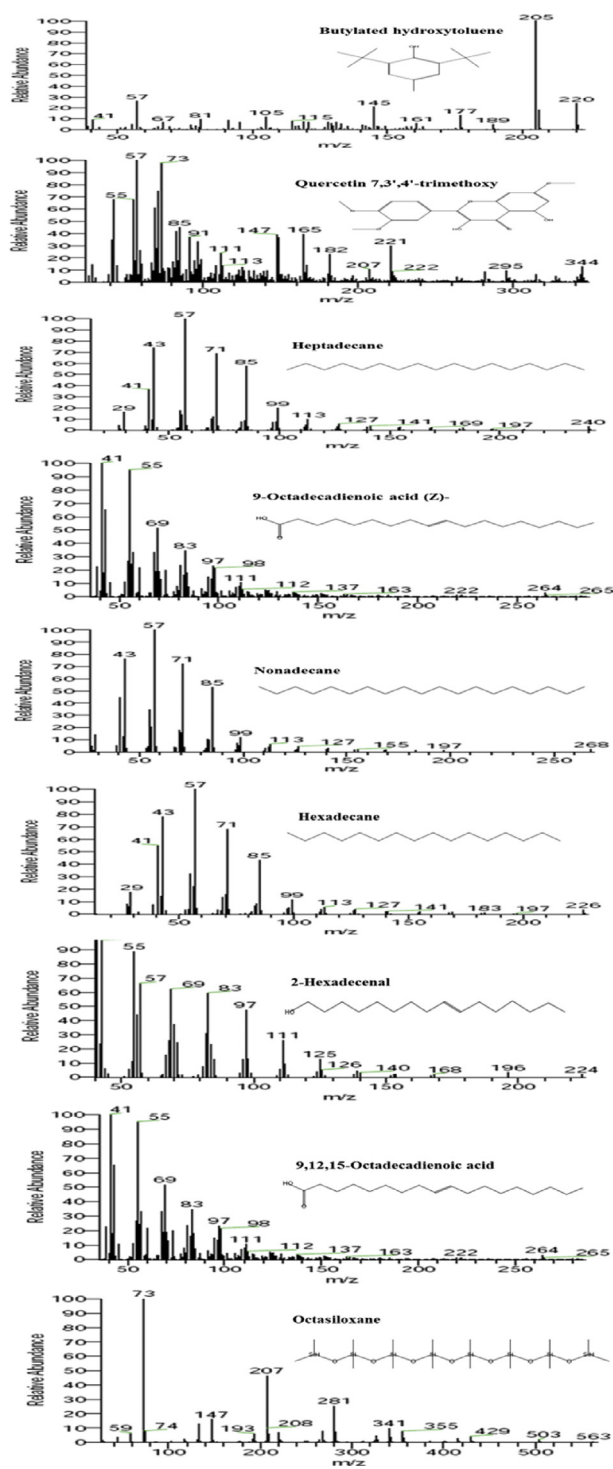
Fig. 5. Mass Spectra of identified compounds in F1 and F7.
