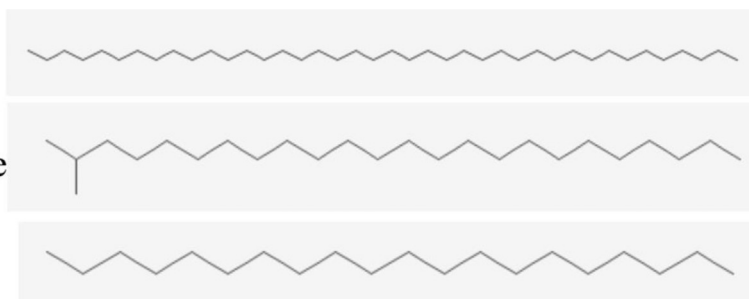
Fig. 5. GC-MS identification of major chemical compounds and their structures of acetone extract of T. asiatica .
