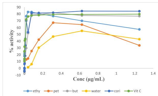
Fig. 2. \text{IC}_{50} values of DPPH radical scavenging activity of extracts and compound from R. heudelotii .
