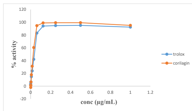
Fig. 3. \text{IC}_{50} values of ABTS activities of corilagin from R. heudelotii .
