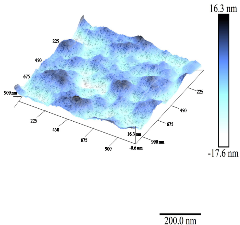
Fig. 8. 2D and 3D AFM images of Ni-W alloy electrodeposits obtained from the bath containing 3,4-Dihydroxybenzaldehyde (250 ppm).
