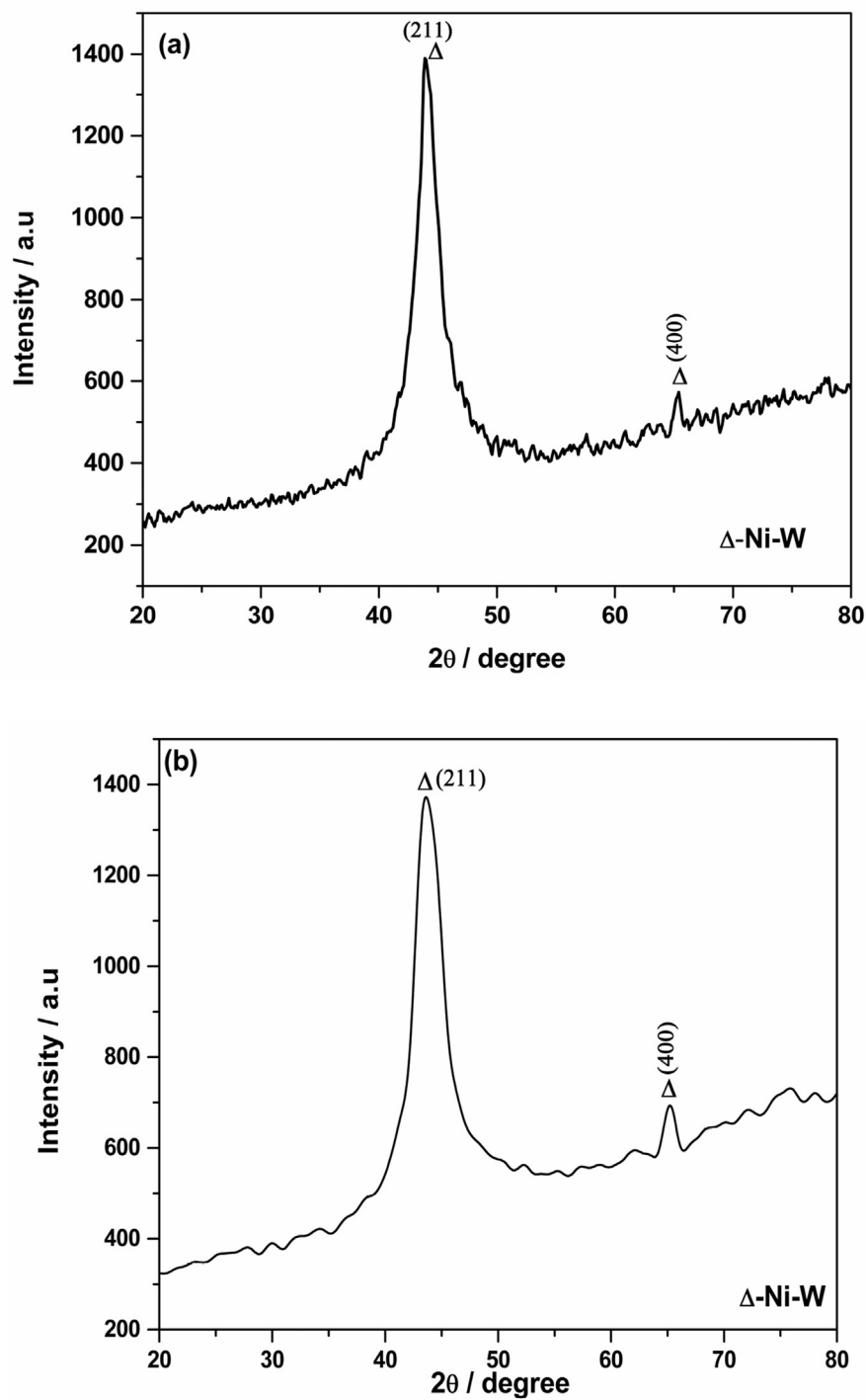
Fig. 4. X-ray diffraction data for Ni-W alloy coatings of as deposited and with that of 3,4-Dihydroxybenzaldehyde (250 ppm) in the plating bath.
