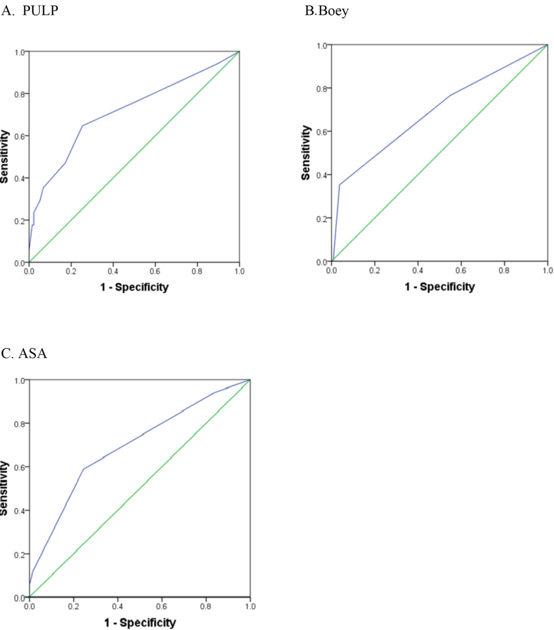
Fig. 1. ROC curves for PULP, Boey and ASA showing the area under the curve.
