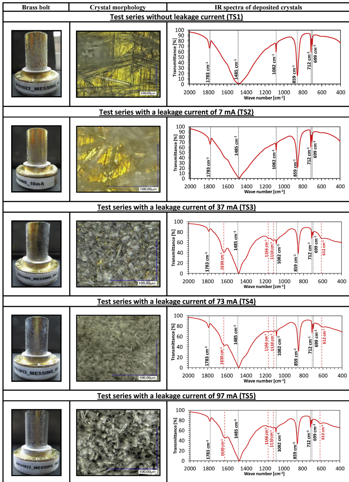
Fig. 13. Contaminated brass bolt, crystal morphology and IR spectra of deposited crystals in dependence on the leakage current.
