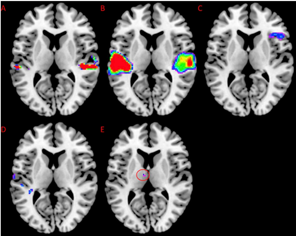
Fig. 3. All results are FWE, p < .05 , > 10 voxels. A and B shows activation following phonetic stimuli in those with right ( n = 12 ) and left ( n = 10 ) SSD. C shows a comparison of activity in the two patient groups (Right SSD – Left SSD). D shows the correlation between activity following phonetic stimuli and the mean sum score for the SAC in all patients. E shows the correlation between the quiet / adverse ratio from the SAC and activity following phonetic stimuli.
