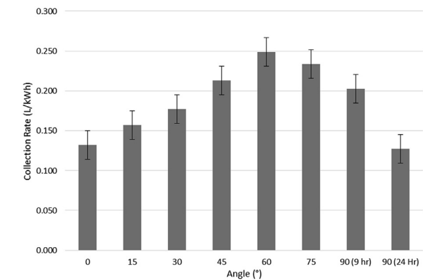
Fig. 10. Average collection rates for the rotated heatsink experiments.
