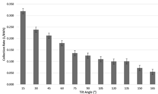
Fig. 20. Average collection rates for the flat plate PTFE surface tilted from 15° to 165° in 15° intervals.
