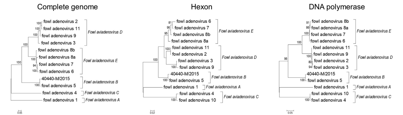
Fig. 3. Phylogenetic analysis of strain 40440-M/2015, a putative new fowl adenovirus type within species Fowl aviadenovirus B . The analyses were conducted based on three stretches: complete genome sequences and derived amino acid sequences of the entire hexon and the DNA polymerase.
