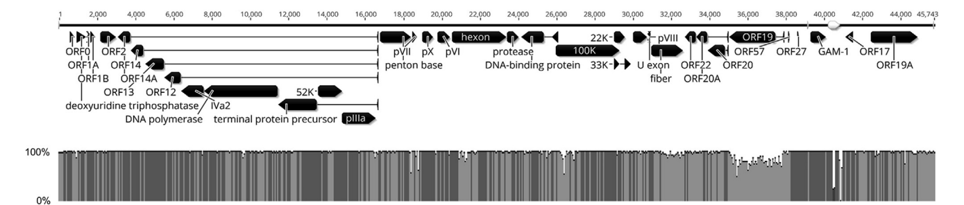
Fig. 2. Genome layout of strain 40440-M/2015, a putative new fowl adenovirus type within species Fowl aviadenovirus B , and its sequence identity to strain 340 (FAdV-5, KC493646). Black arrows in the genome map represent protein coding sequences, white arrows represent repeat regions.
