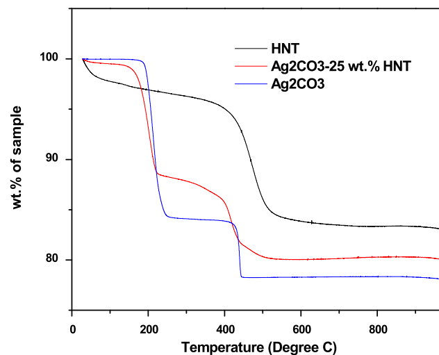
Fig. 4. The thermogravimetric analysis of HNTs, \text{Ag}_2\text{CO}_3 and \text{Ag}_2\text{CO}_3 -HNTs.
