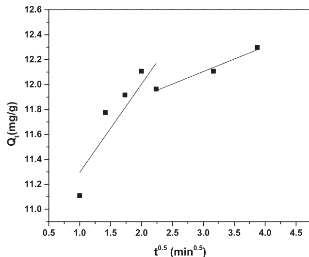
Fig. 13. Interparticle diffusion model for the adsorption of methylene blue unto \text{Ag}_2\text{CO}_3 -50wt.% HNTs.
