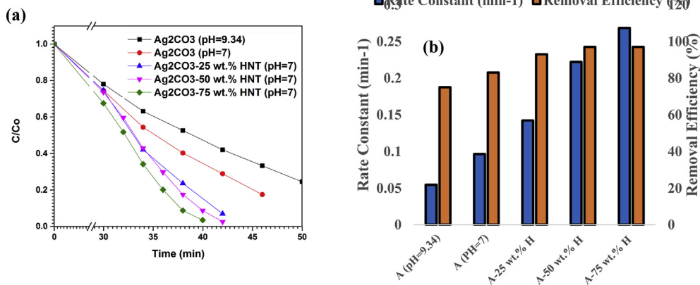
Fig. 6. (a) Photodegradation of rhodamine b dye by \text{Ag}_2\text{CO}_3 and \text{Ag}_2\text{CO}_3 -HNTs (b) Calculated removal efficiencies and first order rate constant ( k ) of \text{Ag}_2\text{CO}_3 and \text{Ag}_2\text{CO}_3 -HNTs [A = \text{Ag}_2\text{CO}_3 , H=HNTs].
