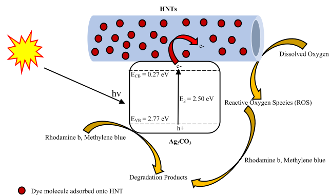
Fig. 11. Schematic diagram for the adsorption and photodegradation of methylene blue and rhodamine B dyes by \text{Ag}_2\text{CO}_3 -HNTs.
