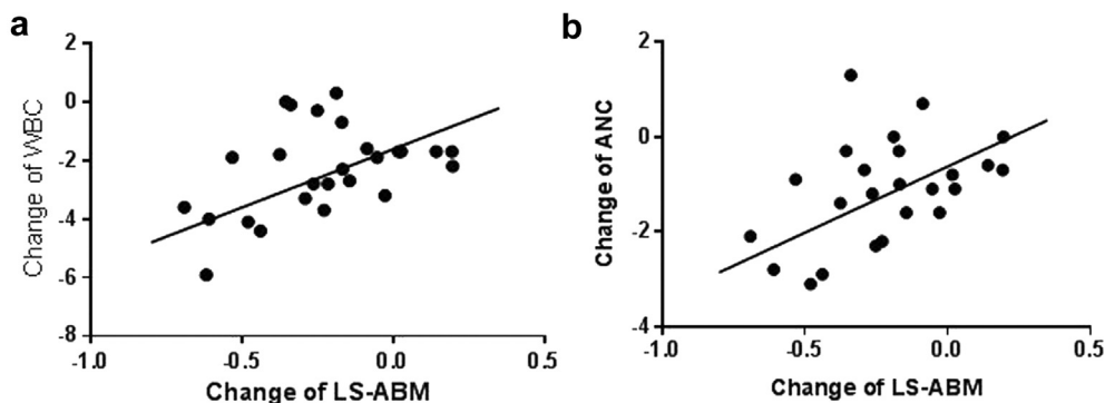
Figure 3 Hematologic toxicity as a function of changes of lumbar-sacral pelvic active bone marrow. (a) Post-chemoradiation therapy change in white blood cell count is linearly correlated to lumbar-sacral pelvic change in active bone marrow ( P = .033 ); and (b) post-chemoradiation therapy change in absolute neutrophil count as a function of lumbar-sacral pelvic change in active bone marrow ( P = .029 )
