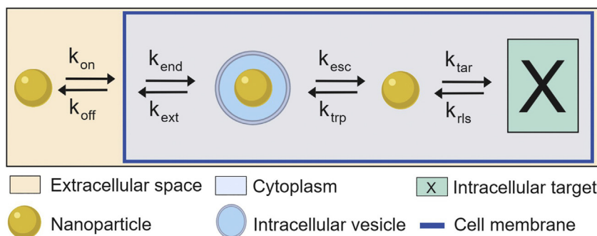
Fig. 10. Compartmental overview diagram depicting major nanoparticle cellular interactions and intracellular transport pathways. Nanoparticles in the extracellular space interact with the cell plasma membrane ( k_{on} , k_{off} ) to enter cells ( k_{end} ). After successful cellular entry, nanoparticles then need to escape ( k_{esc} ) intracellular vesicles (e.g., endosomes) to engage with intracellular targets ( k_{tar} ). Cytoplasmic nanoparticles can be trapped back in vesicular structures ( k_{trp} ) or released from intracellular targets ( k_{rls} ). The excretion of nanoparticles to the extracellular space is defined by k_{ext} . 'k' denotes rate constants for each of these individual steps.
