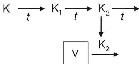
Fig. 11. Schematic overview of pharmacokinetic-pharmacodynamic transit compartment model. 'K' is the initial cell kill rate constant, 'K 1 ' and 'K 2 ' are the cell kill rate constants in the transit compartments, t is the mean transit time, and V is the cell viability. The initial cell kill rate constant is a nonlinear function of nuclear doxorubicin concentration. Adapted with permission from Ref. [247] Copyright (2016) American Chemical Society.
