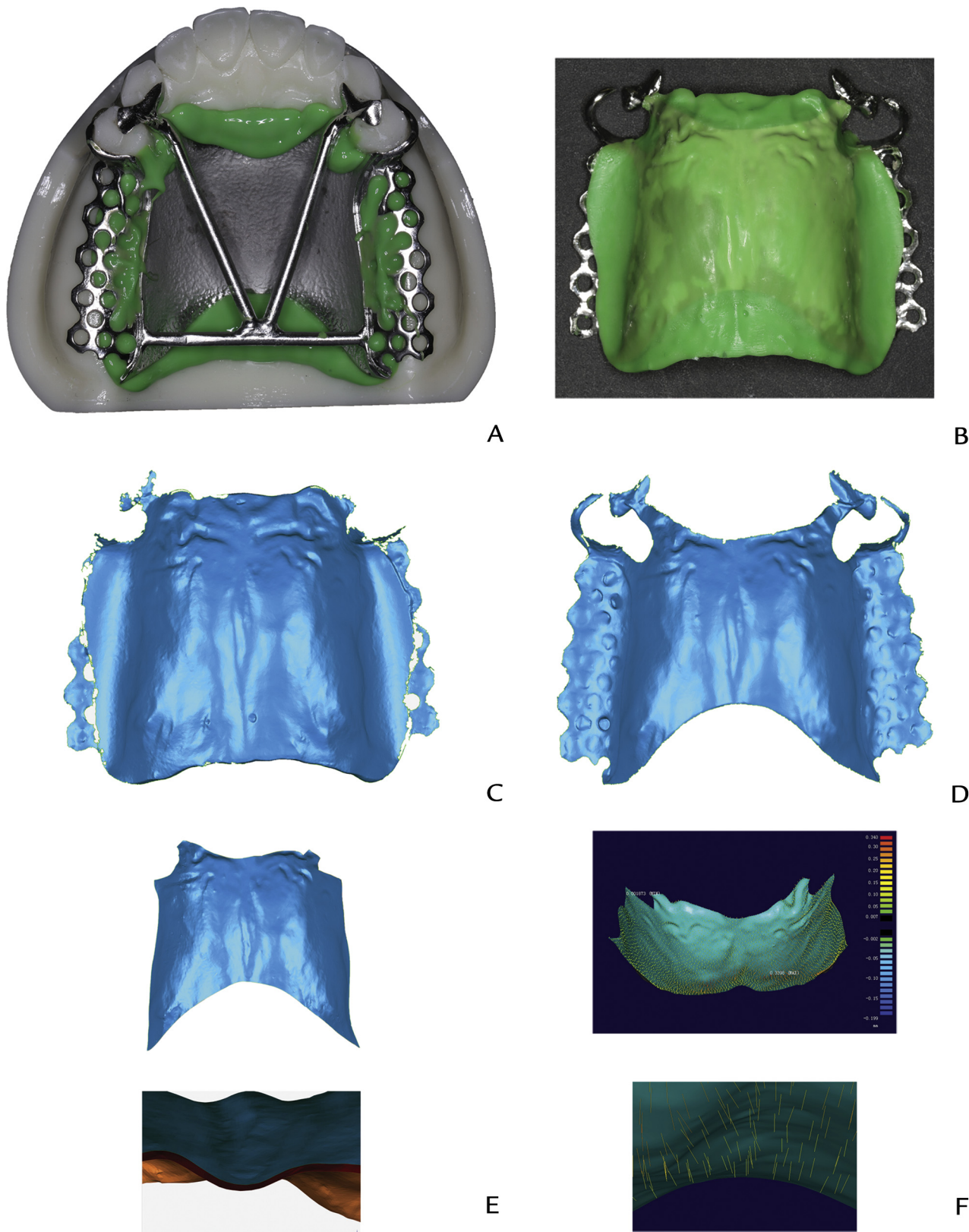
Figure 3. Detection of adaptation of frameworks. A, Frameworks placed on resin models with polyvinyl siloxane impression material. B, Frameworks and impression material remained after removing resin model. C, Surfaces of impression scanned. D, Tissue surfaces of framework scanned after removing impression material. E, Scanned meshes trimmed in Geomagic software, showing gaps between impression surface and framework surface. F, Distances between points on impression surface and mesh surface of framework measured with Imageware software.
