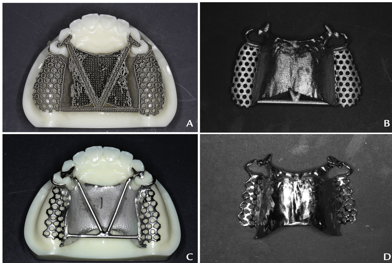
Figure 2. Fabricated removable partial denture frameworks. A, Made by SLM 3D printing. B, Tissue surface of A. C, Made by lost-wax casting. D, Tissue surface of C. SLM, selective laser melting.
