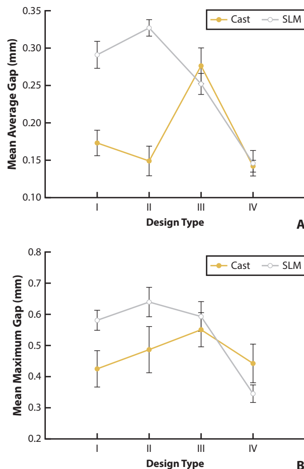
Figure 4. Influence of production methods and design types. A, Mean average gaps. B, Mean maximum gaps. Error bar indicates \pm 1 standard error. SLM, selective laser melting.
