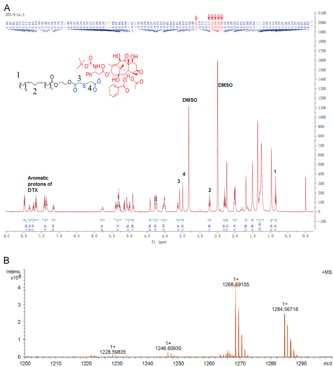
Figure 1 (A) The ^1\text{H} NMR spectra of DTX-S-LA. (B) The MS spectra of DTX-S-LA.
