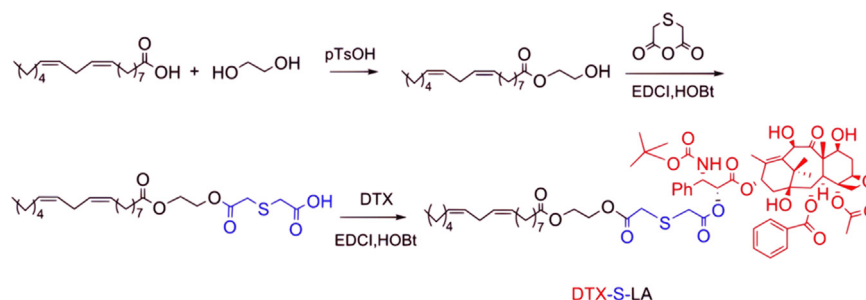
Scheme 1 The synthetic route of DTX-S-LA.
