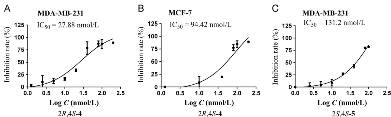
Figure 4 Cytotoxic stereoisomers of 4 and 5 .
