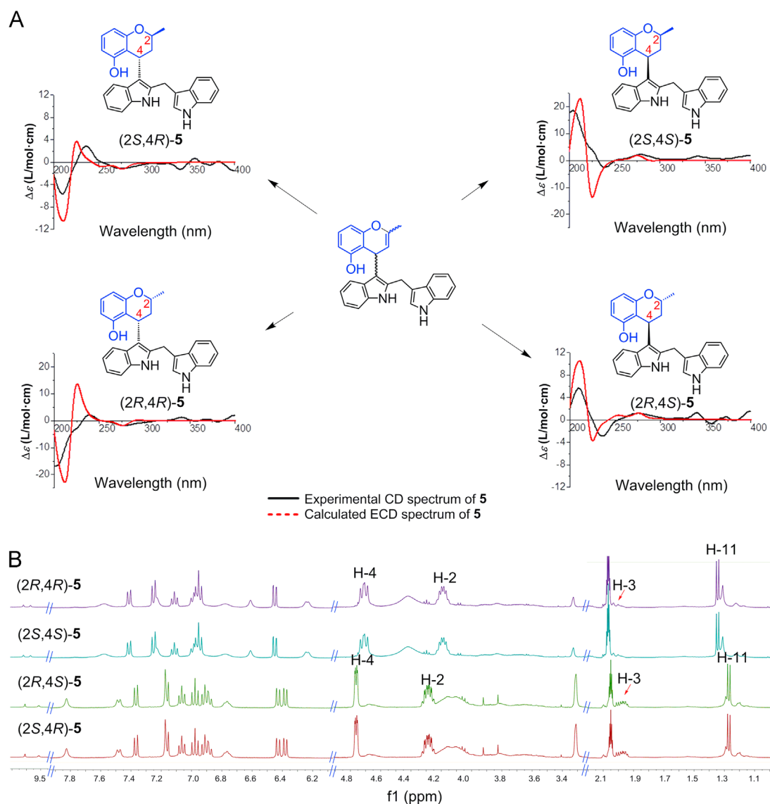
Figure 3 Stereoisomers of indolchromin B ( 5 ). (A) Stereochemical assignment for the major [(2 S ,4 R )- 5 and (2 R ,4 S )- 5 ] and minor [(2 R ,4 R )- 5 and (2 S ,4 S )- 5 ] enantiomer pairs by comparing each recorded CD spectrum with those computed for all options. (B) The difference between the ^1\text{H} NMR spectra of major and minor stereoisomer pairs.
