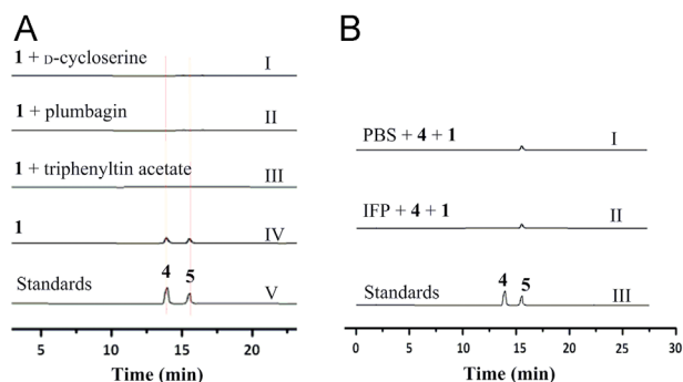
Figure 5 Construction pathways of indolchromins A ( 4 ) and B ( 5 ). (A) AONS is involved in the indolchromin production since 4 and 5 became undetectable if the I3C supplemented fungal culture was exposed additionally to any of the AONS inhibitors D-cycloserine (I), plumbagin (II) and triphenyltin acetate (III) at 1.0 mmol/L. (B) Non-enzymatic formation of 5 from 4 via incorporating 3-MEI [freshly derived from I3C ( 1 ), see Scheme 1].
