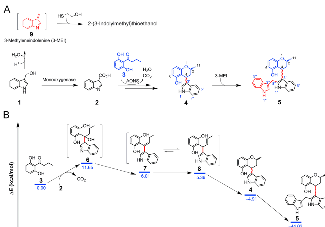
Scheme 1 Indolchromins A ( 4 ) and B ( 5 ) resulting from the coupling of fungal polyketide with I3C ( 1 ) catabolites. (A) Proposed polyketide-indole hybridization leading to 4 and 5 in the I3C exposed fungal culture. (B) Reaction energy profile for the generation of 4 and 5 computed by DFT method at B3LYP/6-31+G(d,p) level in polarizable continuum model (PCM, dielectric constant \epsilon = 78.39 for H 2 O). The relative energies in kcal/mol are calculated from the sums of the respective total energies ( E_{\text{sol}} ) of all species (Supporting Information Table S2). AONS, 8-amino-7-oxononanoate synthase; I3CA ( 2 ), indole-3-carboxylic acid.
