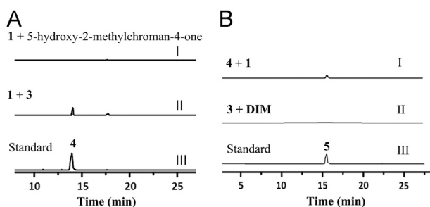
Figure 6 Identification of the precursor of indolchromins A ( 4 ) and B ( 5 ). (A) Compound 4 was formed by co-exposing 1 and 3 to the intracellular fungal protein (IFP), but failed to be detected if IFP was mixed with 1 and 5-hydroxy-2-methylchroman-4-one. (B) Compound 5 was generated when exposing IFP to 4 and 1 (as a 3-MEI precursor), but not produced if IFP was mingled with 3 and DIM.
