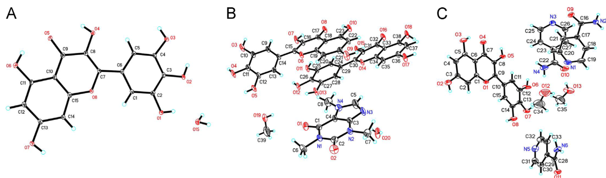
Figure 12 The atoms number of the asymmetric unit for MYR·H 2 O (A), MYR-CAF·MeOH (B) and MYR-INM·2MeOH cocrystals (C).
