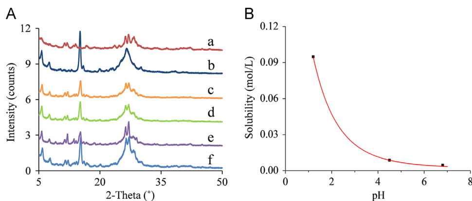
Figure 10 PXRD patterns of the residual solid after equilibrium solubility studies (A) of MYR (a) and MYR-INM (b) performed in buffer solution (37 °C) with pH 6.8 (c), pH 4.5 (d), pH 1.2 (e), and water (f). Thermodynamic solubility–pH dependence of 1:3 MYR-INM cocrystal (B). Black squares represent the measured cocrystal solubilities at transition points. Red curve was generated using models that describe cocrystal solubility–pH dependence according to Eq. (3) and the parameter values were presented in Table 1.
