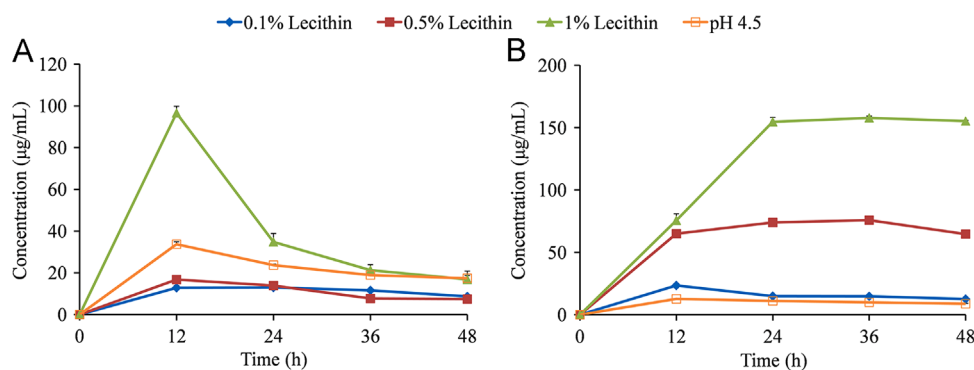
Figure 7 Apparent solubility of MYR-INM (A) and MYR-CAF (B) cocrystals in the pH 4.5 buffer containing 0.1% Lecithin (♦), 0.5% Lecithin (■), 1% Lecithin (▲), or blank pH 4.5 buffer (□) ( n = 3 ).
