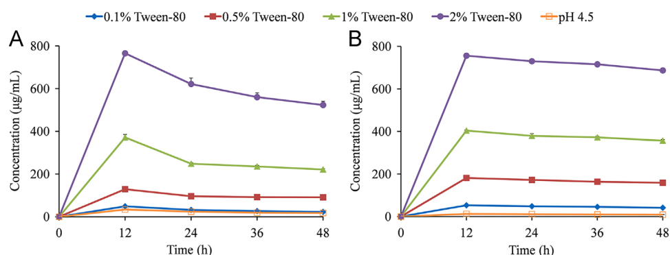
Figure 8 Apparent solubility of MYR-INM (A) and MYR-CAF (B) cocrystals in the pH 4.5 buffer containing 0.1% Tween-80 (♦), 0.5% Tween-80 (■), 1% Tween-80 (▲), 2% Tween-80 (●), or blank pH 4.5 buffer (□) ( n = 3 ).
