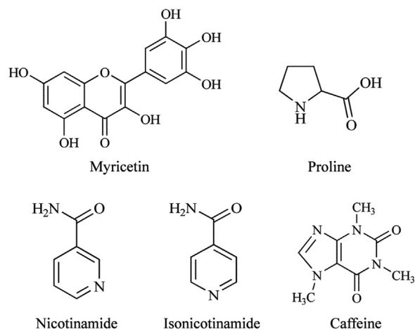
Figure 1 Chemical structures of myricetin (MYR) and cocrformers.
