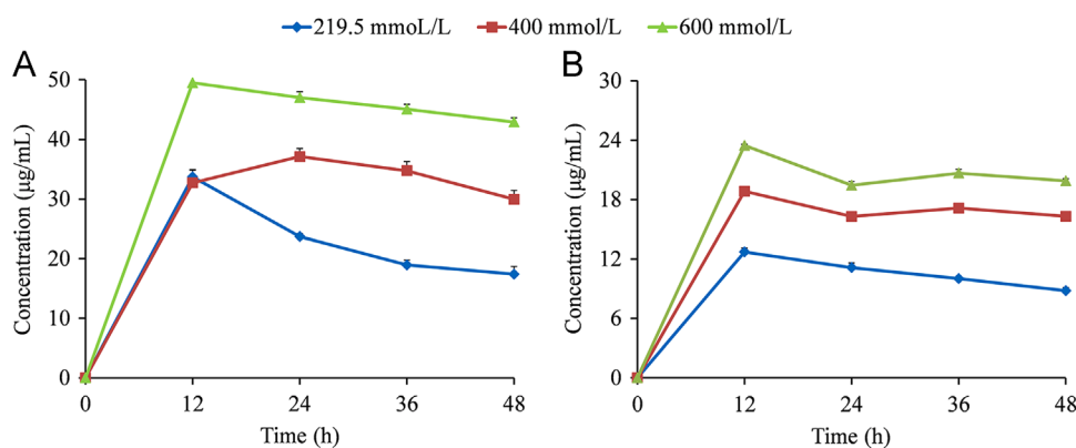
Figure 9 Apparent solubility of MYR-INM (A) and MYR-CAF (B) cocrystals in 219.5 mmol/L (◆), 400 mmol/L (■), 600 mmol/L (▲) ( n = 3 ).
