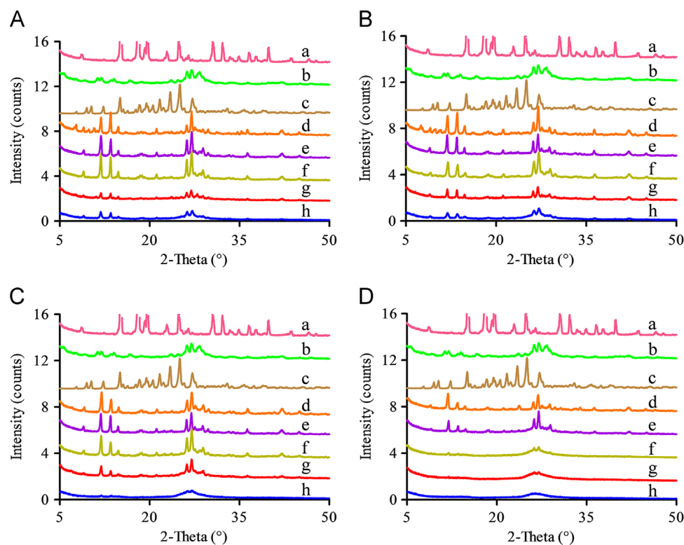
Figure 4 PXRD patterns of the residual solid obtained from the apparent solubility of MYR-PRO cocrystal, which was performed in water (A) and buffer solutions of pH 1.2 (B), pH 4.5 (C), and pH 6.8 (D) at 4 h (h), 6 h (g), 12 h (f), 24 h (e), 48 h (d), respectively. The PXRD patterns of the corresponding PRO (a), MYR (b), and MYR-PRO cocrystal (c) were also given to confirm the composition of the residual solid.
