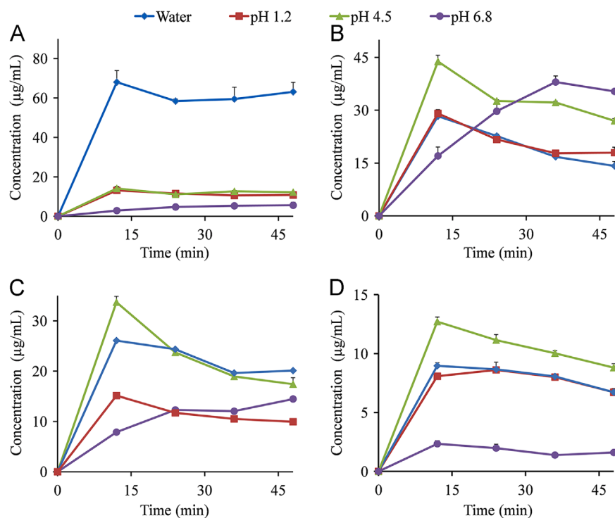
Figure 2 Dynamic solubility profiles for MYR-PRO (A), MYR-NIC (B), MYR-INM (C), and MYR-CAF (D) cocrystals in water (♦) and aqueous solution at pH 1.2 (■), pH 4.5 (▲), pH 6.8 (●) ( n = 3 ).
