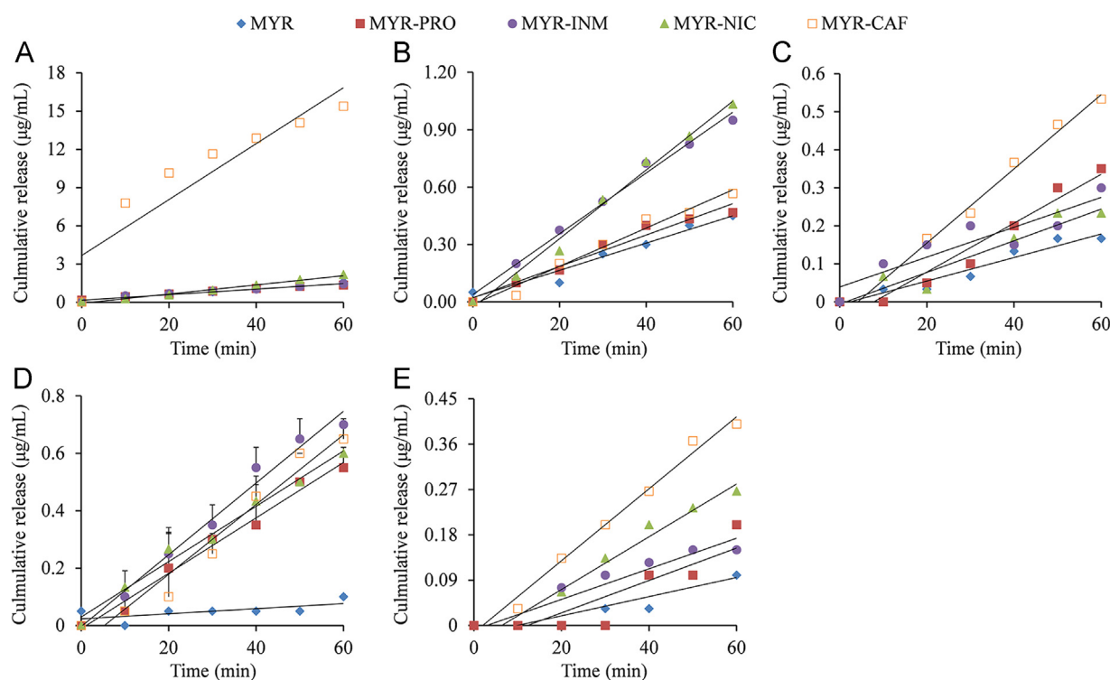
Figure 11 IDR profiles (first 60 min shown) at of MYR (♦), MYR–PRO cocrystal (■), MYR–INM cocrystal (●), MYR–NIC cocrystal (▲), and MYR–CAF cocrystal (□) performed in 0.5% Tween-80 (A), water (B), and buffer solution of pH 1.2 (C), pH 4.5 (D), pH 6.8 (E) at 37 °C ( n = 3 ).
