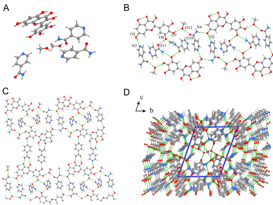
Figure 15 Unit cell (a), 1D chain (b), 2D sheet (c), 3D structure (d) for MYR-INM·2MeOH cocrystal.
