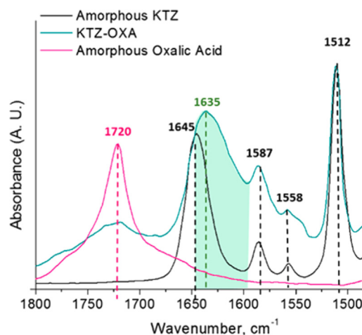
Figure 4 IR spectra of amorphous ketoconazole (KTZ), coamorphous ketoconazole (KTZ)–oxalic acid (OXA) and amorphous oxalic acid (OXA). (Adapted from the Ref. 77 with the permission. Copyright © 2018 American Chemical Society).
