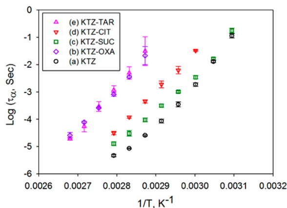
Figure 5 Temperature dependence of \alpha -relaxation times of (a) amorphous ketoconazole (KTZ), (b) coamorphous KTZ-oxalic acid (OXA), (c) KTZ-succinic acid (SUC), (d) KTZ-citric acid (CIT), and (e) KTZ-tartaric acid (TAR). (Adapted from the Ref. 77 with the permission. Copyright © 2018 American Chemical Society).
