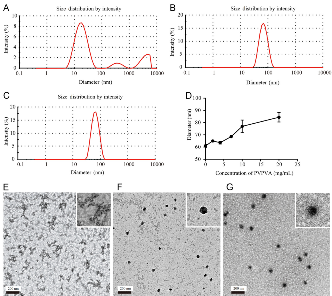
Figure 4 Size distributions of (A) PVPVA; (B) Soluplus; and (C) Soluplus-PVPVA (2:8, v/v) complex measured by dynamic light scattering. (D) Effect of the concentration of PVPVA on the size of Soluplus micelles. Values are expressed as the mean \pm SD, n=3 . TEM photographs of (E) PVPVA, (F) Soluplus and (G) Soluplus/PVPVA (2:8, v/v) complex (scale bar: 200 nm).
