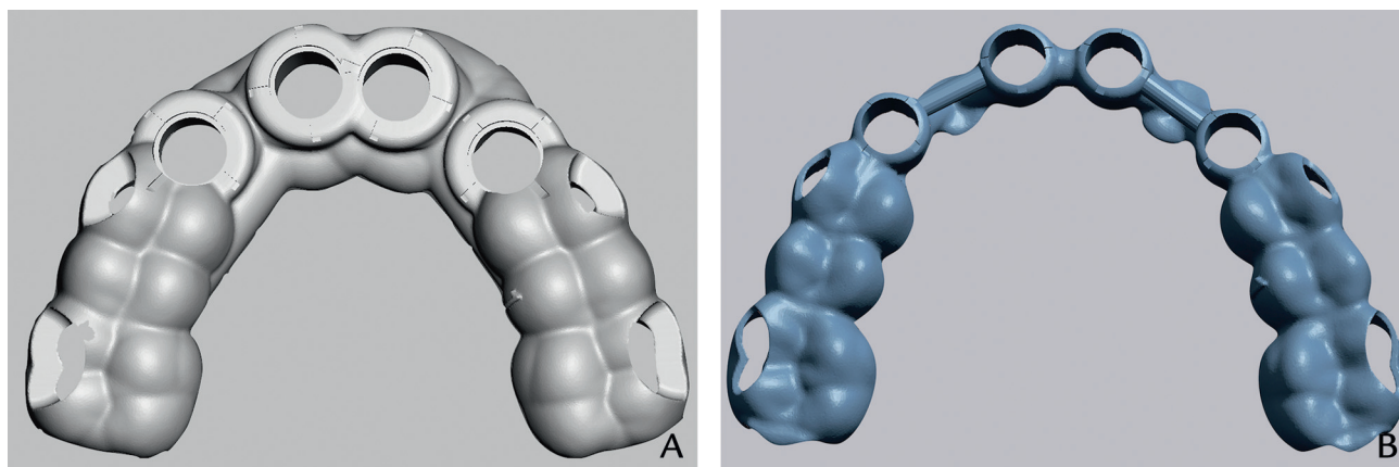
Figure 1. Representative designs of additively manufactured surgical templates. A, Design for SLA and PolyJet for production of resin surgical templates. B, Design for DMP for production of Co-Cr metal surgical templates. DMP, direct metal printing; SLA, stereolithography.
