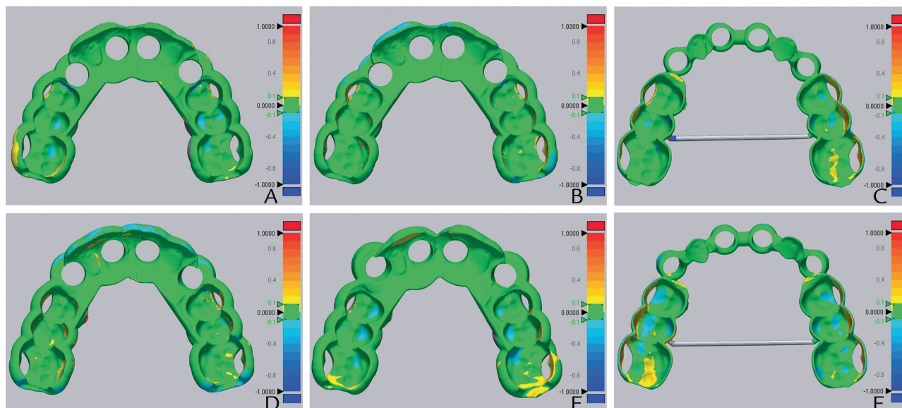
Figure 2. Representative surface matching color maps from 6 study groups. A, SLA immediately. B, PolyJet immediately. C, DMP immediately. D, SLA at 1 month. E, PolyJet at 1 month. F, DMP at 1 month. DMP, direct metal printing; SLA, stereolithography.
