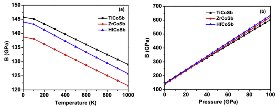
Fig. 2. Plot of bulk modulus with respect to (a) Temperature and (b) Pressure for MCoSb (M = Ti, Zr and Hf).
