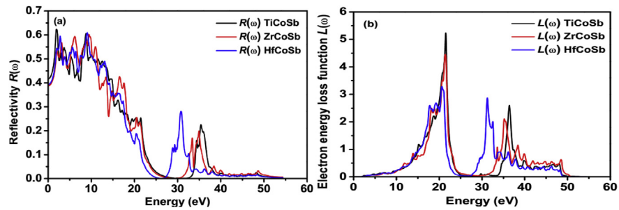
Fig. 5. Plot of (a) Reflectivity R(\omega) and (b) Electron energy loss functional L(\omega) vs Photon energy.
