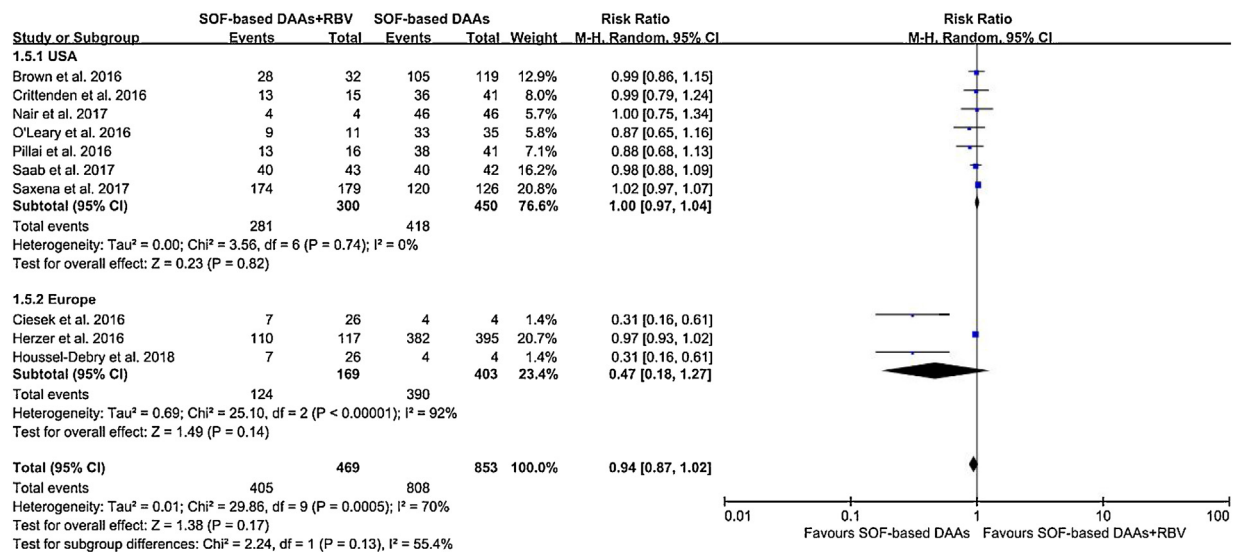
Figure 4. Risk ratio of sustained virological response 12 weeks (SVR12) after the end of treatment in patients with post-liver transplantation in different regions.
