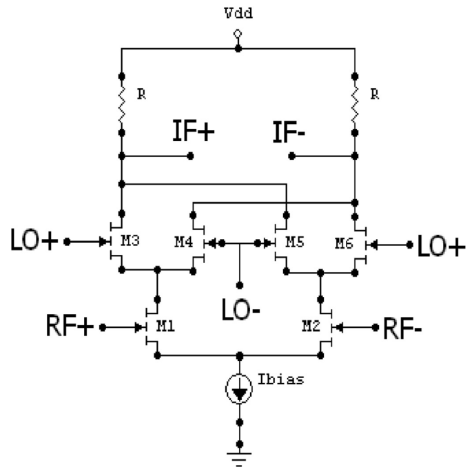
Fig. 3. Double-balanced mixer.
