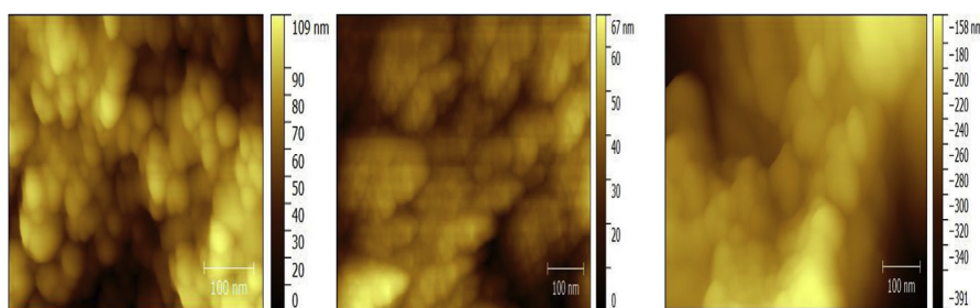
Fig. 3. AFM images of coated \text{TiO}_2 photoelectrodes with P3HT (left), polythiophene network (middle) and polythiophene nanoparticles (right) at 100 °C.
