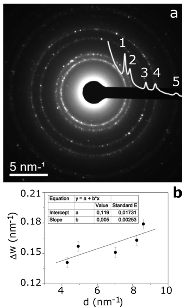
Fig. 4. (a) Diffraction ring showed by an AgNP-PMMA, (b) Williamson-Hall plot obtained from the electron diffraction profile.
