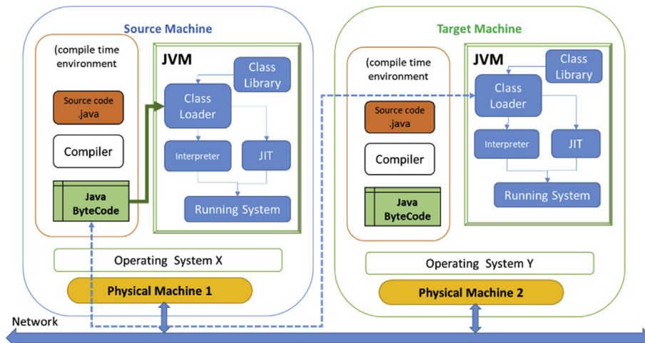
Fig. 3. Java virtual machine task exchange on a loosely-coupled network.
