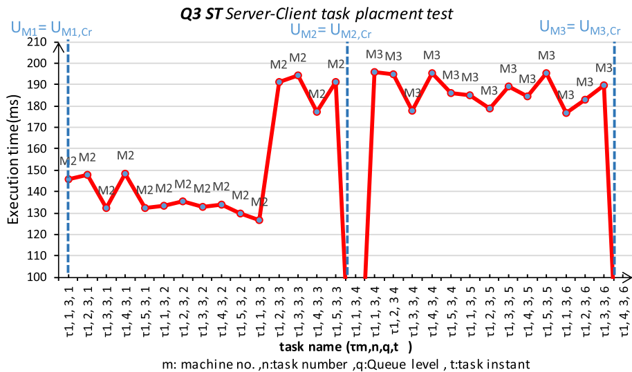
Fig. 15. Server-Client (M1: M2, M3) task placement for “Soft Real-time tasks ST-Q2” for load-balance on M1.
