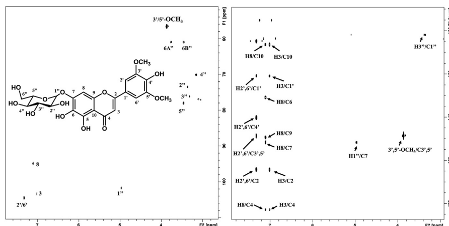
Fig. 2. Expanded regions of the HSQC spectrum (left) and HMBC spectrum (right) of 5,6,7,4'-tetrahydroxy-3',5'-dimethoxy-flavone 7-O- \beta -D-glucopyranoside ( 2 ) with assigned crosspeaks.
