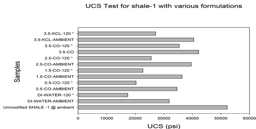
Fig. 9. Uniaxial compressive strength (UCS) test for shale-1.
