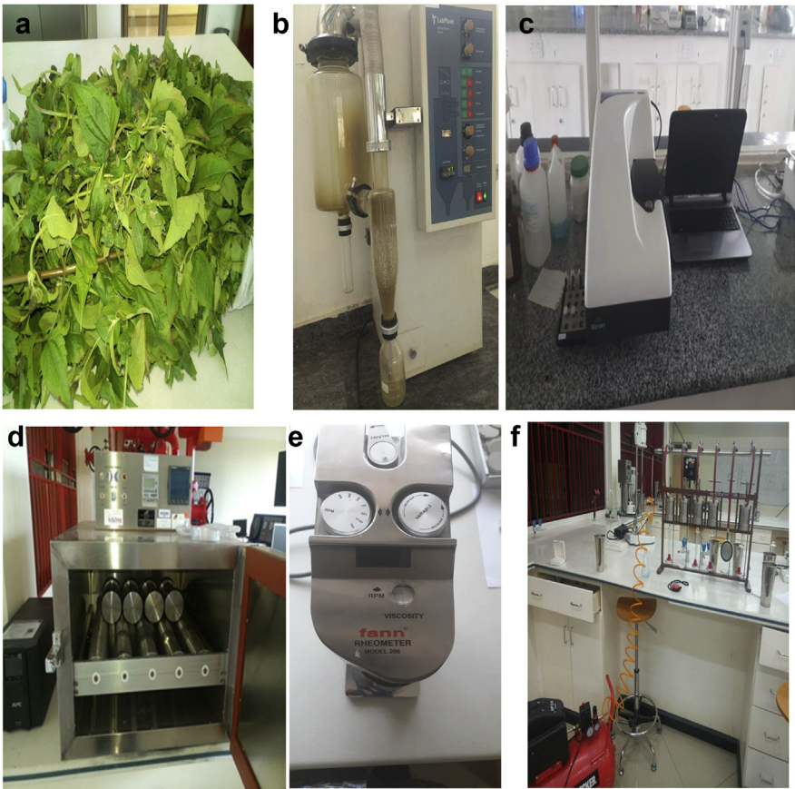
Fig. 1. a) Chromolaena odorata Leaf Collected for Analysis. b) Lab Plant SD-05 Spray Dryer used for test. c) Malvern Zetasizer Nano ZS90. d) 5-Speed Hot Roller Oven. e) FANN Rheometer model. f) API Low Pressure Multiple Filter Press.
