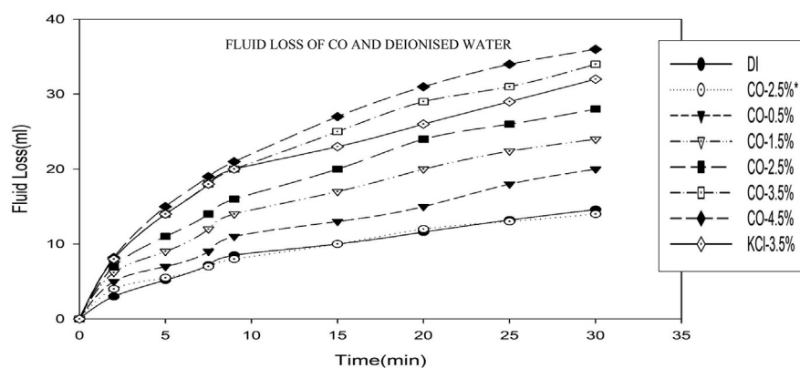
Fig. 5. Filtration (Fluid Loss) for CO, KCl and De-Ionised Water (DI).
