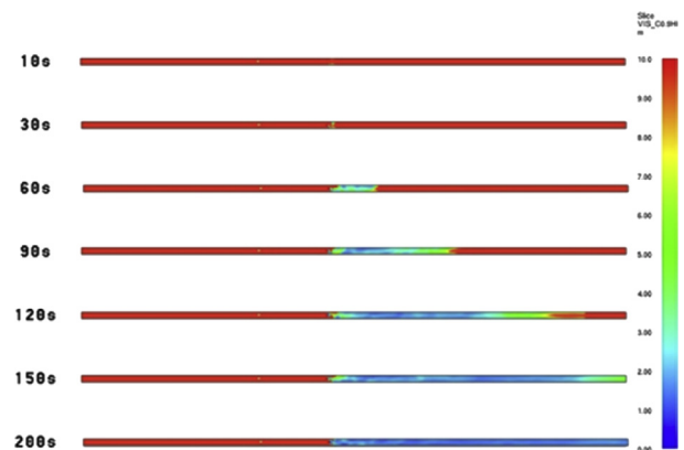
Fig. 14. Vision contour at 2 m above the tunnel floor in the presence of the jet fan.
