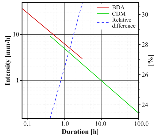
Fig. 11. Comparison between the CDM- and the BDA-based rainfall thresholds for the study area and their relative difference respect the BDA values.
