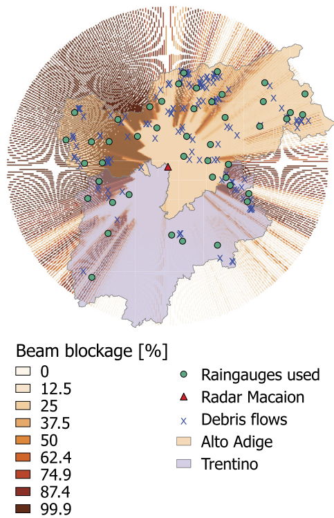
Fig. 6. Percentage of signal attenuation due to beam blocking effect on the debris flows considered with radar beam elevation at 1^\circ .
