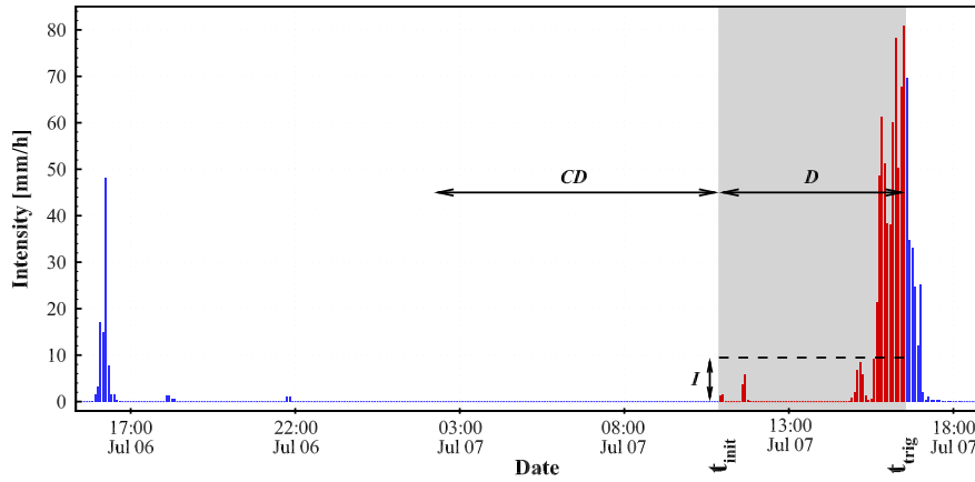
Fig. 1. Example of determination the rain relevant to a real debris flow. Here, t_{trig} \equiv t_{max} , t_{init} is obtain by using the CDM, D = t_{trig} - t_{init} and I is the event-averaged rain intensity.
