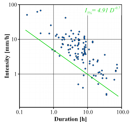
Fig. 8. The CDM-based rainfall threshold for the study area.
