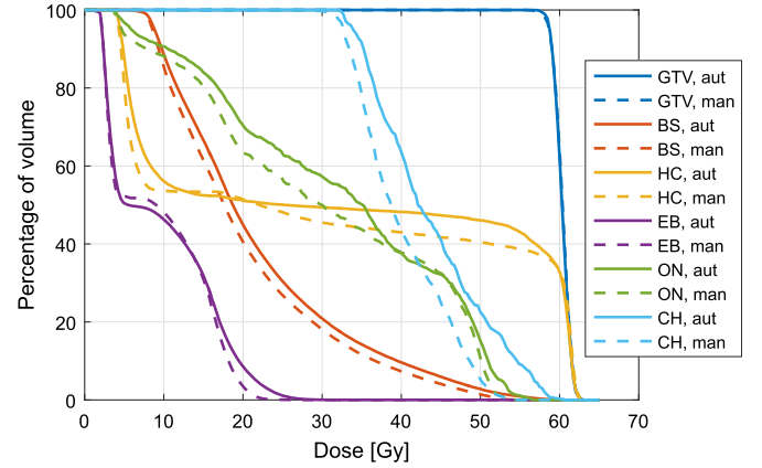
Fig. 10. Dose volume histogram (DVH) of several structures for the representative subject in Fig. 9, i.e., tumor core (GTV), brainstem (BS), hippocampi (HC), eyes (EB), optic nerves (ON), and chiasm (CH). Solid lines and broken lines correspond to automatic and manual segmentations, respectively. Note that all DVHs were computed using the original treatment dose plan, which was based on the manual segmentations.
