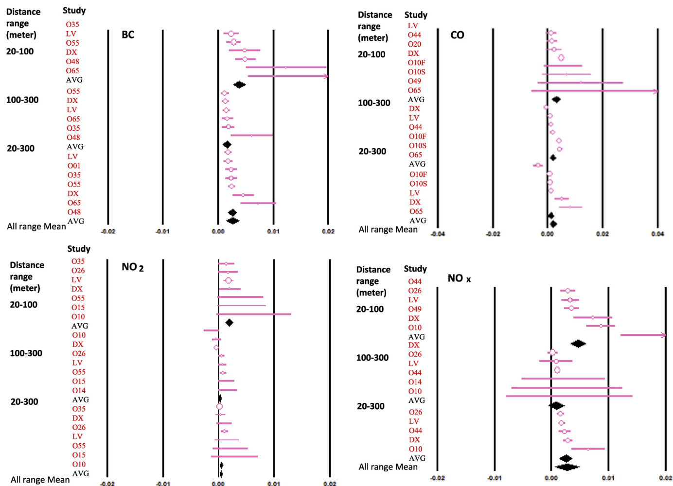
Fig. 1. Meta-data analysis of decay rates for selected traffic-related air pollutants. The different types of air pollutants are shown in separate plots for Black carbon (BC), carbon monoxide (CO), nitrogen dioxide (NO 2 ) and nitrogen oxides (NO x ), respectively. A red line with open circle represents the 95% confidence intervals (CI) and the mean each individual study. Diamond under each set of distance range represents the average of a meta-analysis for that distance range. The diamond aligned with “All range mean” at the bottom of each plot refers to meta-analysis on all three ranges for a given pollutant. Study IDs are as explained in Table 3.
