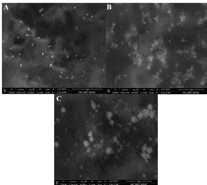
Fig. 8. SEM images of synthesized silver nanoparticles at different neem leaf broth concentration (A) 5%, (B) 10%, (C) 15%.
