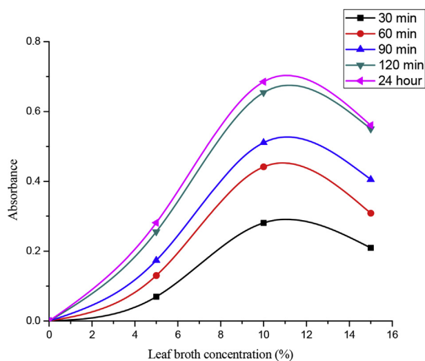
Fig. 7. Time course of AgNPs synthesis with different leaf broth concentration (5%–15%), \text{AgNO}_3 = 1 \times 10^{-3} \text{ mol dm}^{-3} , temperature = 30 °C.
