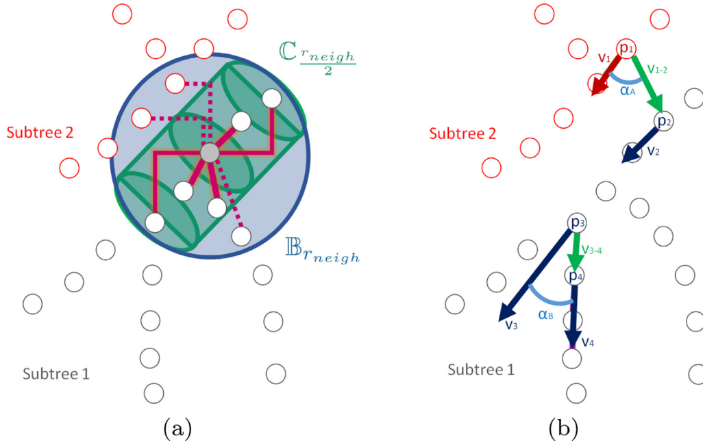
Fig. 5. a) Anisotropic connection strategy using a cylindrical confinement (green) along the preferential local direction of vessels impede inter-irrigation connections (dashed lines) between vessel particles (circles) that could be connected when using an isotropic strategy (blue area). b) Connectivity vector between particles can improve the definition of edge weights based on parallelism between preferential directions. Intertwined structures could report unreal parallelism between preferential directions ( v_1 and v_2 ) of particles belonging to different irrigations ( p_1 and p_2 ) that can be minimized using the direction of connectivity vector ( v_{1-2} ). The instability in the definition of preferential directions ( v_3 ) in bifurcations ( p_3 ) may mask real coorientations ( p_3 and p_4 ) that can be enhanced using the connectivity vector ( v_{3-4} with v_4 ). For interpretation of the references to color in this figure legend, the reader is referred to the web version of this article.
