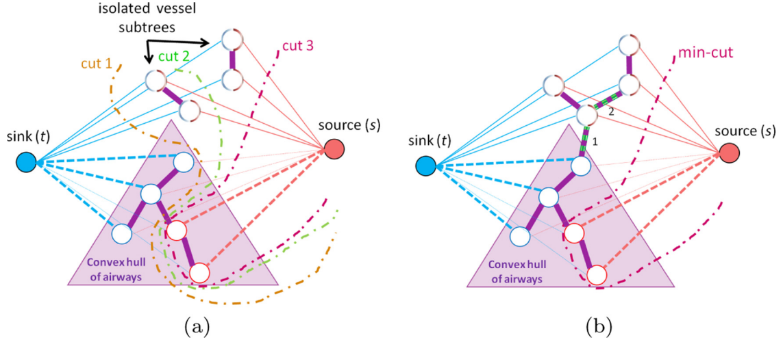
Fig. 6. a) Example of a forest with three connected components showing two isolated subtrees located outside the convex hull of airways (purple area). Consequently, the three cuts displayed need the same energy to be performed, rendering their selection as min-cut equally probable. b) Refinement of the graph results on the addition of new edges 1 and 2 (purple-green dashed lines) and the uniqueness of min-cut. For interpretation of the references to color in this figure legend, the reader is referred to the web version of this article.
