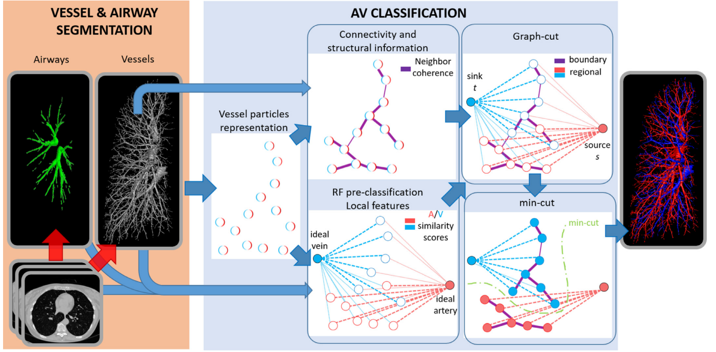
Fig. 2. Graphical scheme of the proposed framework for the automatic AV segmentation algorithm. AV classification is performed over a set of scale-space vessel particles coming from the initial segmentation. Connectivity and structural information is used to compute neighbour coherence, forming the boundary term ( n -links, purple lines); and RF pre-classification based on local features extracted from vascular and bronchial information is used to compute arterial/venous similarity scores, forming the regional term ( t -links, red/blue links) of the graph-cut. The final AV classification is obtained by computing the minimum-cut. Circles depict vessel particles, thickness of connections represent the weight of the links, and circumference colors show the preferential class for each particle. For interpretation of the references to color in this figure legend, the reader is referred to the web version of this article.
