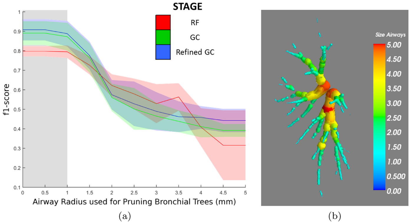
Fig. 11. Importance of airways segmentation in AV results. a) Evolution of F1-scores when pruning airway segmentations by removing particles with scales lower than a specific value. Mean values (lines) and standard deviations (shadows) are displayed for the three evaluation stages. b) Example of an airway tree where the scale of particles at each bronchial location is represented.
