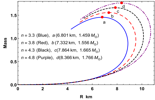
Fig. 13. Variation of mass with R assuming a = 0.004 and b = 0.01^{n-1} for the range 3.3 < n < 5 .
