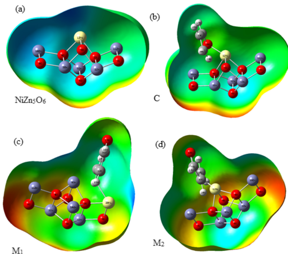
Figure 6. Molecular electrostatic potential surfaces for (a) \text{NiZn}_5\text{O}_6 (b) C interaction site of A- \text{NiZn}_5\text{O}_6 (c) \text{M}_1 interaction site of A- \text{NiZn}_5\text{O}_6 (d) \text{M}_2 interaction site of A- \text{NiZn}_5\text{O}_6 calculated at B3LYP/6-31G level of theory.
