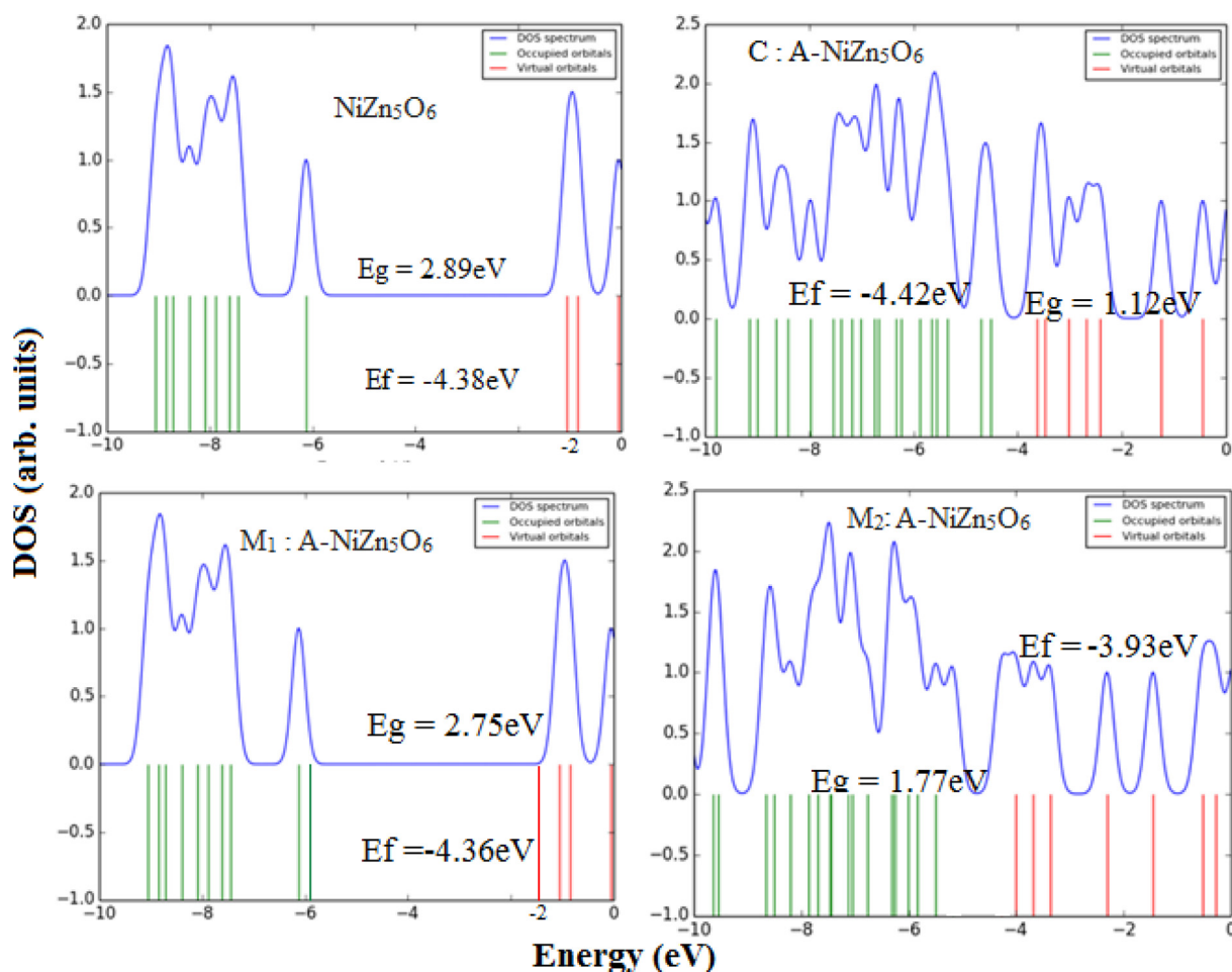
Figure 4. The DOS plot of (a) \text{NiZn}_5\text{O}_6 (b) C interaction site of \text{A-NiZn}_5\text{O}_6 (c) \text{M}_1 interaction site of \text{A-NiZn}_5\text{O}_6 (d) \text{M}_2 interaction site of \text{A-NiZn}_5\text{O}_6 .
