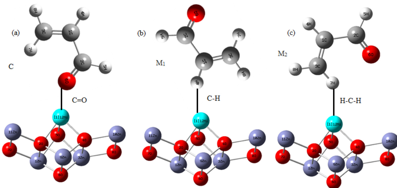
Figure 2. The adsorption of acrolein on Ni doped Zn 6 O 6 with (a) C (Carbonyl) (b) M 1 (Methyl) (c) M 2 (Methylene) interaction site calculated at B3LYP/6-31G level of theory.
