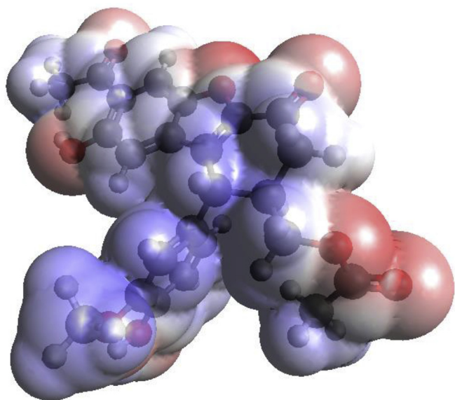
Fig. 3. Calculated MEP pattern of propolisbenzofuran B molecule at B3LYP/6-311++G(d,p) computational level.
