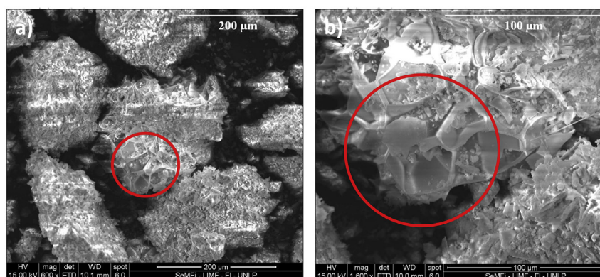
Fig. 7. Precipitate formed in the EC process a) 600X b) 1600X.
