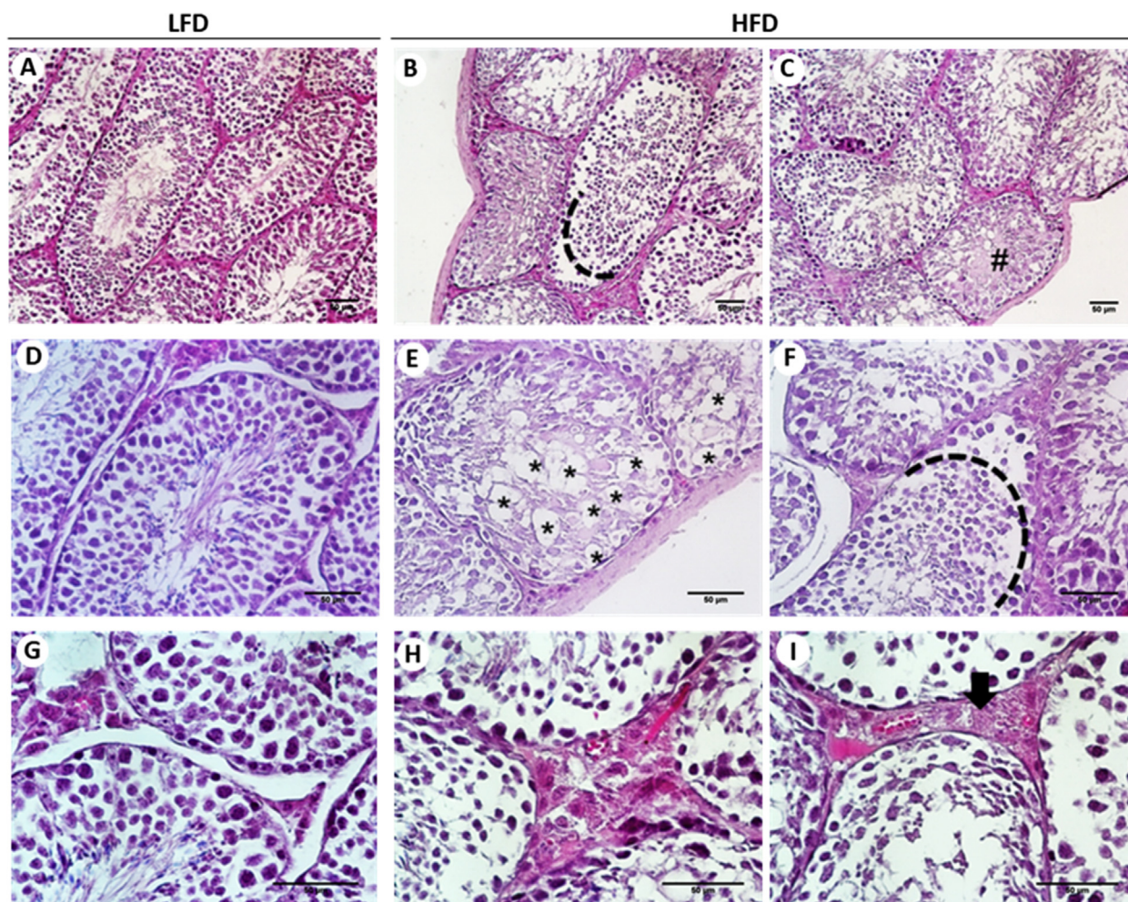
Fig. 2. HFD altered testicular morphology in C57BL/6J mice. Representative H&E images of LFD testicular tissue exhibit a normal histological morphology. Testicles from HFD mice show loosely arranged spermatogenic cells (dashed lines) on the seminiferous epithelium, epithelial disruption (#), vacuoles in the testis (*) and enlarged interstitium (black arrows). Magnification: A, B and C, 200 X; D, E and F, 400 X; and G, H and I, 600 X.
