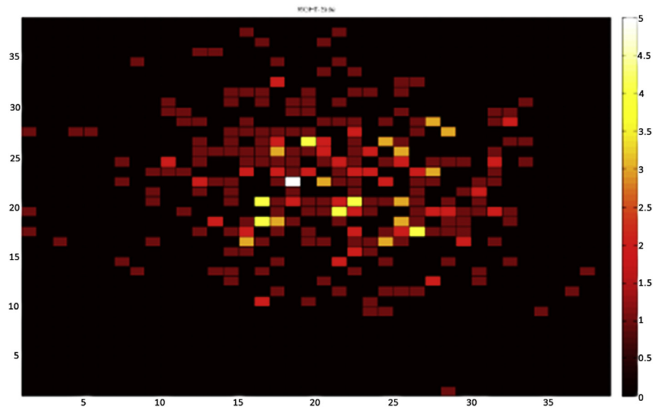
Fig. 6. The Probability Density Function (PDF) of the values of each slice. The frequency position is color coded on the right hand side heat map bar.
