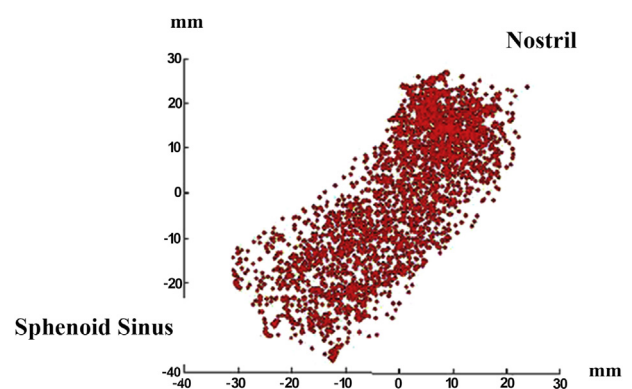
Fig. 7. Workspace of EETS showing the spatial.
