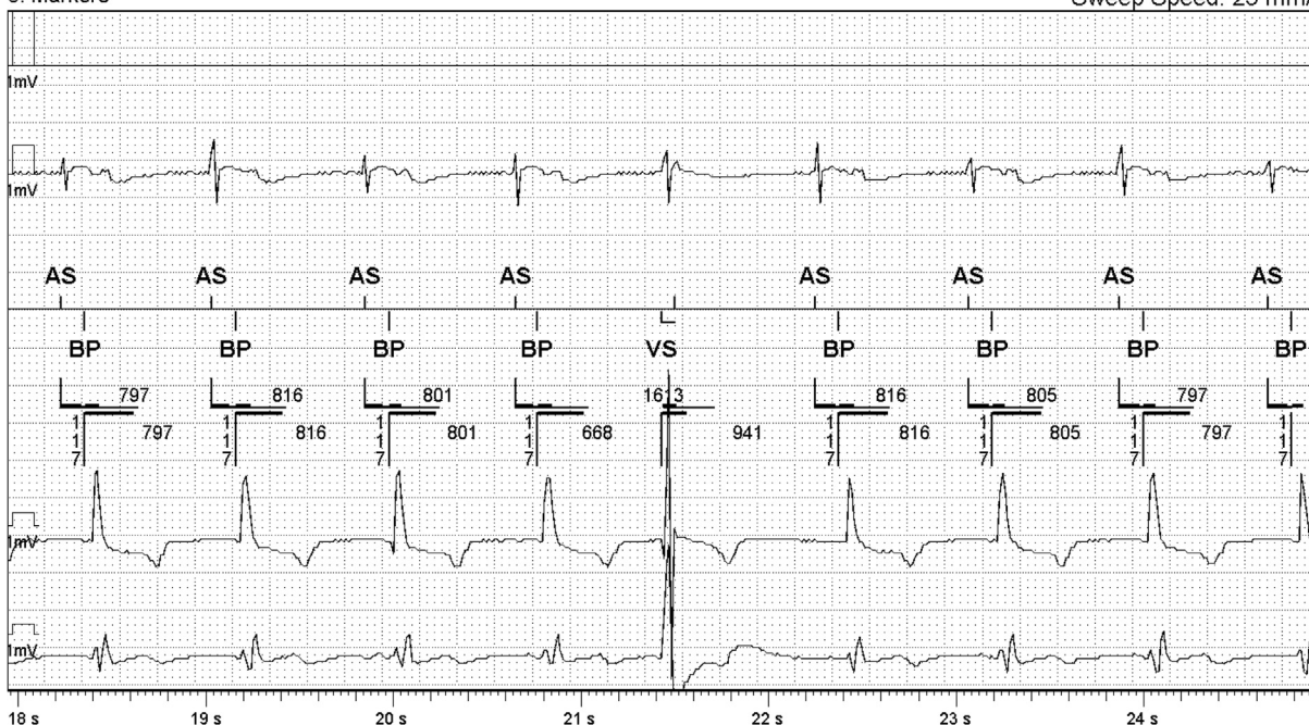
Figure 2 After the atrial pace premature ventricular contraction (PVC) response algorithm was disabled, PVCs occurred without closely coupled atrial pacing. Of note, the intrinsic atrial activity early in the extended postventricular atrial refractory period likely would be too early to result in long-short induced atrial fibrillation even if the PVC response had remained on. LV = left ventricle; RV = right ventricle.
