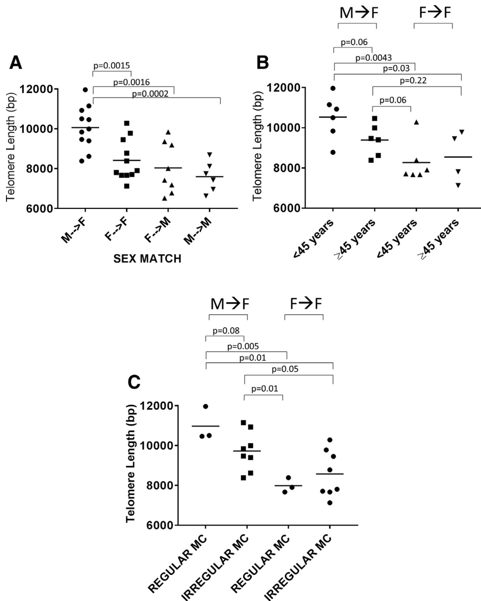
Figure 2. Determinants of TL in UCBT patient cohort. (A) Dot plot graphs showing longest TL in male to female (M→F) UCBT compared with all other subgroups (M→F n = 11; F→F n = 11; F→M n = 8; M→M n = 6). Differences between groups were calculated using the Student t -test. A P < .05 was considered as statistically significant. The bars represent the mean values. Observed power (alpha = .05): M→F versus F→F, .96; M→F versus F→M, .97; M→F versus M→M, .99. (B) Dot plot graph showing that TL was significantly longer in young (<45 years of age) female recipients receiving male UCB compared with those receiving female UCBs. Furthermore, there was a trend toward longer telomeres in young female compared with older female UCBT recipients receiving a male UCB graft (45 years is the median age of M→F transplant recipients). On the contrary, no such a trend in favor of younger recipients was observed in female to female transplants. (M→F < 45 n = 6; M→F ≥ 45 n = 6; F→F < 45 n = 6; F→F ≥ 45 n = 4). Observed power (alpha = .05): <45 M→F versus <45 F→F, .95; <45 M→F versus ≥45 M→F, .58; <45 M→F versus ≥45 F→F, .77; ≥45 M→F versus <45 F→F, .60; ≥45 M→F versus ≥45 F→F, .32. (C) Dot plot graphs showing longest TL in male UCB transplanted in women with regular menstrual cycles (MC). Among female recipients with regular MC (6/22), male UCBs had significantly longer telomeres compared with female UCBs. (M→F regular MC n = 3; M→F irregular MC n = 8; F→F regular MC n = 3; F→F irregular MC n = 8). Observed power (alpha = .05): M→F regular MC versus M→F irregular MC, .56; M→F regular MC versus F→F regular MC, .99; M→F regular MC versus F→F irregular MC, .90; M→F irregular MC versus F→F regular MC, .84; M→F irregular MC versus F→F irregular MC, .85.
