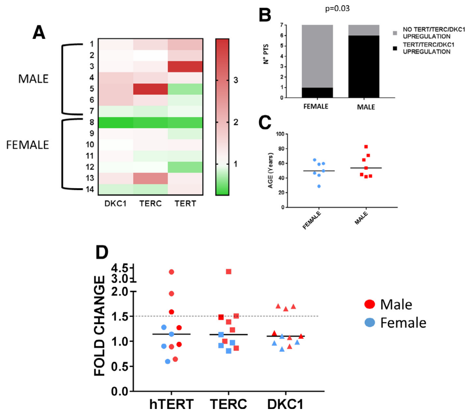
Figure 3. Ex vivo E_2 exposure upregulates telomerase subunits in male-derived bone marrow MNCs. (A) Heat map showing gene expression changes of telomerase subunits genes TERT , TERC , and DKC1 in BM-derived MNCs from 14 subjects (7 men, 7 women) treated with E_2 .1 nM for 24 hours. Gene expression fold changes are shown in a colorimetric scale from green (low) to red (high). Primary BM MNCs from lymphoma patients undergoing initial staging procedures (who then resulted negative for lymphoma bone marrow infiltration) were obtained through density gradient separation, cultured in RPMI medium supplemented with 10% FBS, and treated ex vivo with DMSO (control) or .1 nM E_2 for 24 hours. mRNA was extracted and measured by TaqMan qPCR assays. (B) Bar graph showing the proportion of subjects upregulating at least 1 telomerase subunits (by a fold change \geq 1.5 ) in male versus female subgroups. P value was calculated using the Fisher exact test. (C) Dot plot graph representing age in male (red dots) versus female (blue dots) subjects. Lines represent medians. (D) Dot plot graphs showing fold change of telomerase subunits mRNA levels after E_2 exposure (data shown in A) after postmenopausal female donors ( n = 3 ) were excluded from the analysis. Significant upregulation of telomerase subunits (by a fold change \geq 1.5 ) was observed exclusively in E_2 -treated male-derived BM MNCs.
