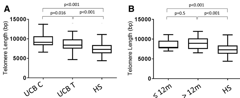
Figure 1. UCBT recipients maintain significantly longer telomeres compared with age-matched healthy control subjects. (A) Box plot graph showing TL of the UCBT recipient cohort (UCB T, n = 36) compared with a control group of UCBs (UCB C, n = 46) and age-matched healthy subjects (HS, n = 85). Differences between groups were calculated using the Student t -test. A P < .05 was considered as statistically significant. NS indicates not significant. Observed power (alpha = .05): UCB C versus UCB T, .76; UCB-T versus HS, .99; UCB C versus HS, .99. The box extends from the 25th to 75th percentiles, bars are min to max values. (B) Box plot graph showing TL of UCBT patients depending on the timing of TL measurement (>12 months, n = 21, versus ≤12 months, n = 15). Observed power (alpha = .05): ≤12 months versus >12 months, .16; ≤12 months versus HS, .85; >12 months versus HS, .93.
