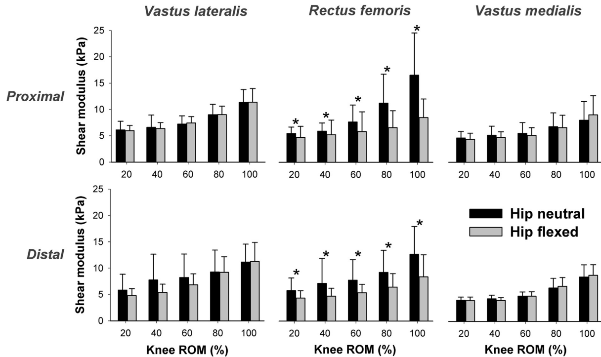
Fig. 2. Shear modulus for each knee range of motion percentile of the proximal and distal regions of vastus medialis, rectus femoris, and vastus lateralis in two hip positions: neutral ( 0^\circ ) and flexed at 80^\circ . Mean \pm SD values are plotted. * Indicates statistical differences between hip positions ( p < 0.05 ).
