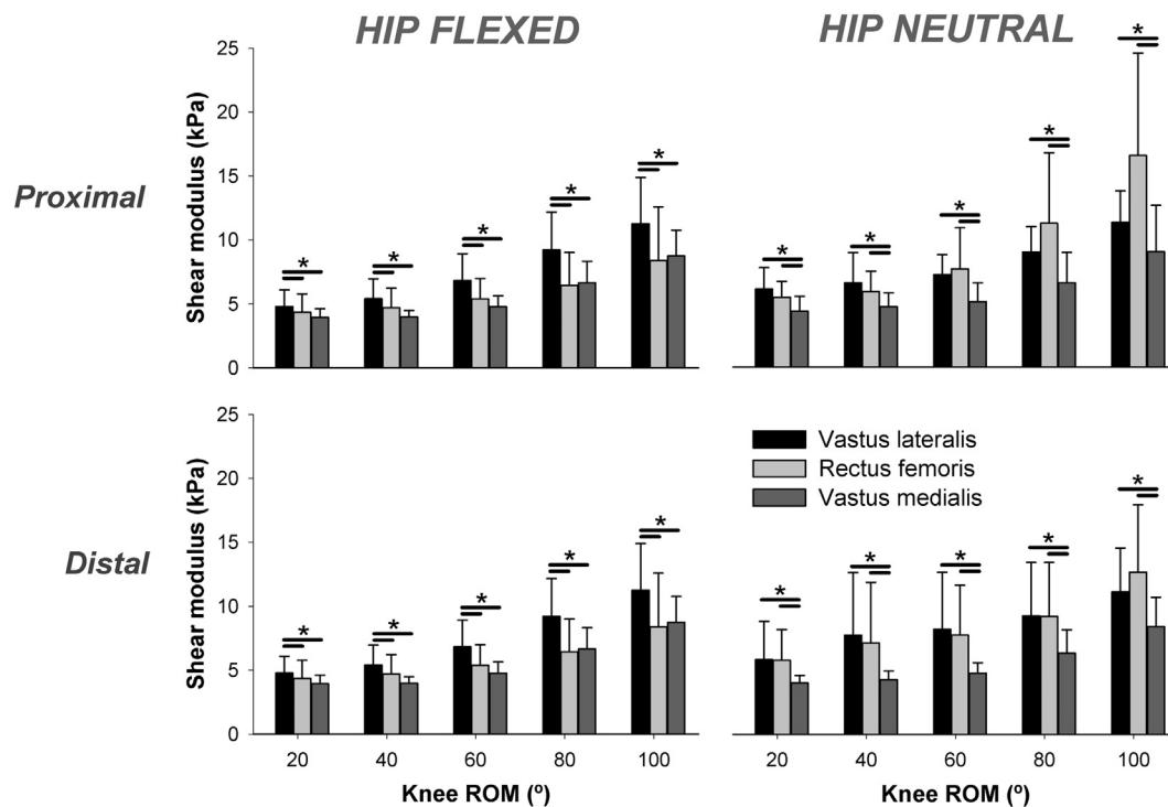
Fig. 3. Shear modulus-range of motion curves for the proximal and distal regions of vastus medialis, rectus femoris, and vastus lateralis in either hip neutral ( 0^\circ ) or flexed ( 80^\circ ) positions. Mean \pm SD values are plotted. Data shown in this figure is the same as for Fig. 2, but differently organized to provide a better, and different, readability. * Indicates statistical differences between muscles ( p < 0.05 ).
