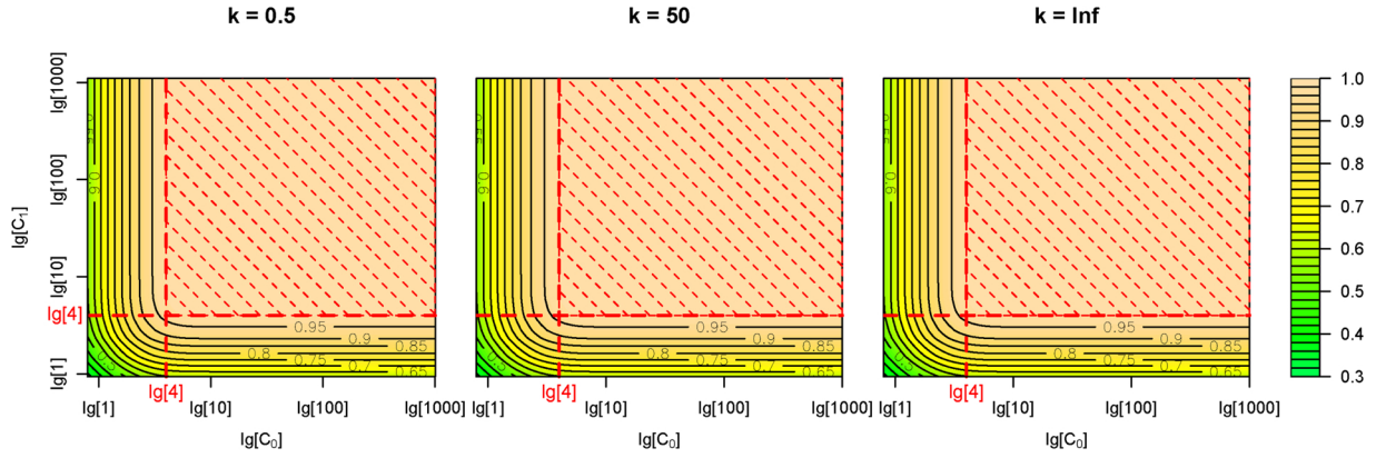
Fig. 1. The heatmap for the probability of at least one event in both the reference group and the treatment group ( C_0 is the expected total number of crashes in the reference group and C_1 is that of the treatment group.)
