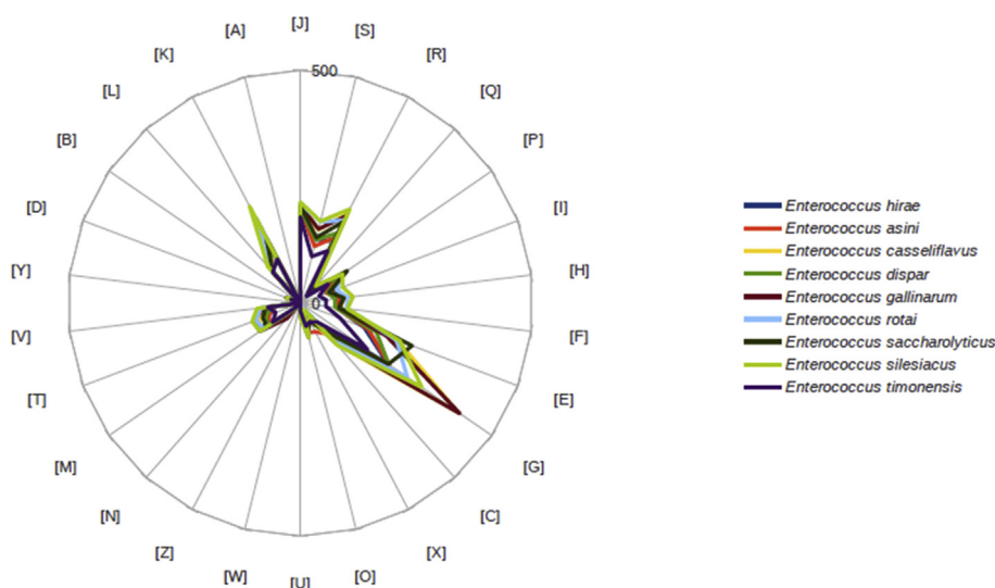
FIG. 6. Distribution of functional classes of predicted genes in genomes from Enterococcus timonensis , E. hirae , E. gallinarum , E. saccharolyticus , E. casseliflavus , E. rotai , E. silesiacus and E. asini chromosomes according to clusters of orthologous groups of proteins.
