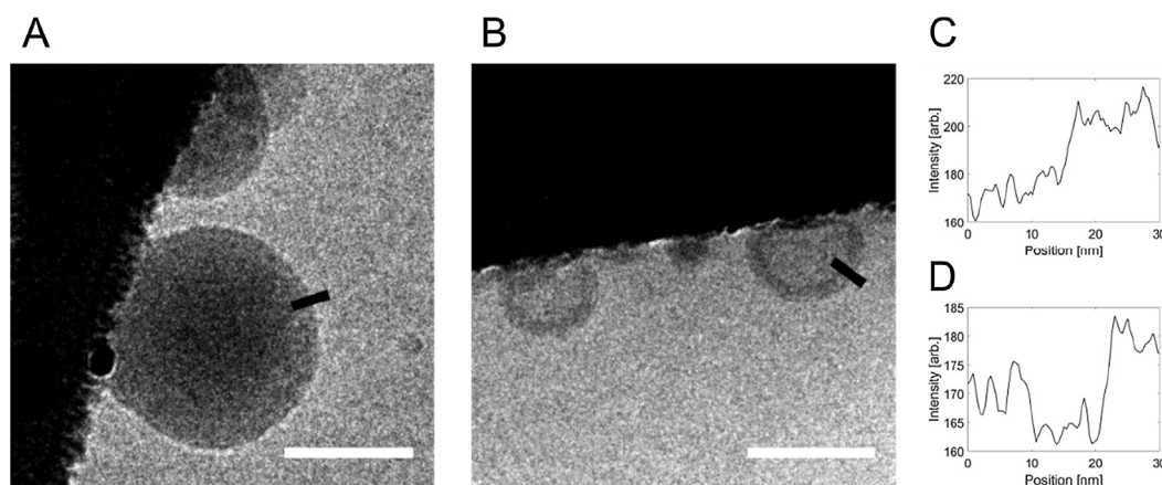
Fig. 1. Representative cryo-TEM images of siRNA-loaded LPNs (A) and SNALPs (B). Electron density profiles across the edge of particles (black lines) show a uniform structure of siRNA-loaded LPNs (C) and a core-shell structure of SNALPs (D). Scale bars = 100 nm.
